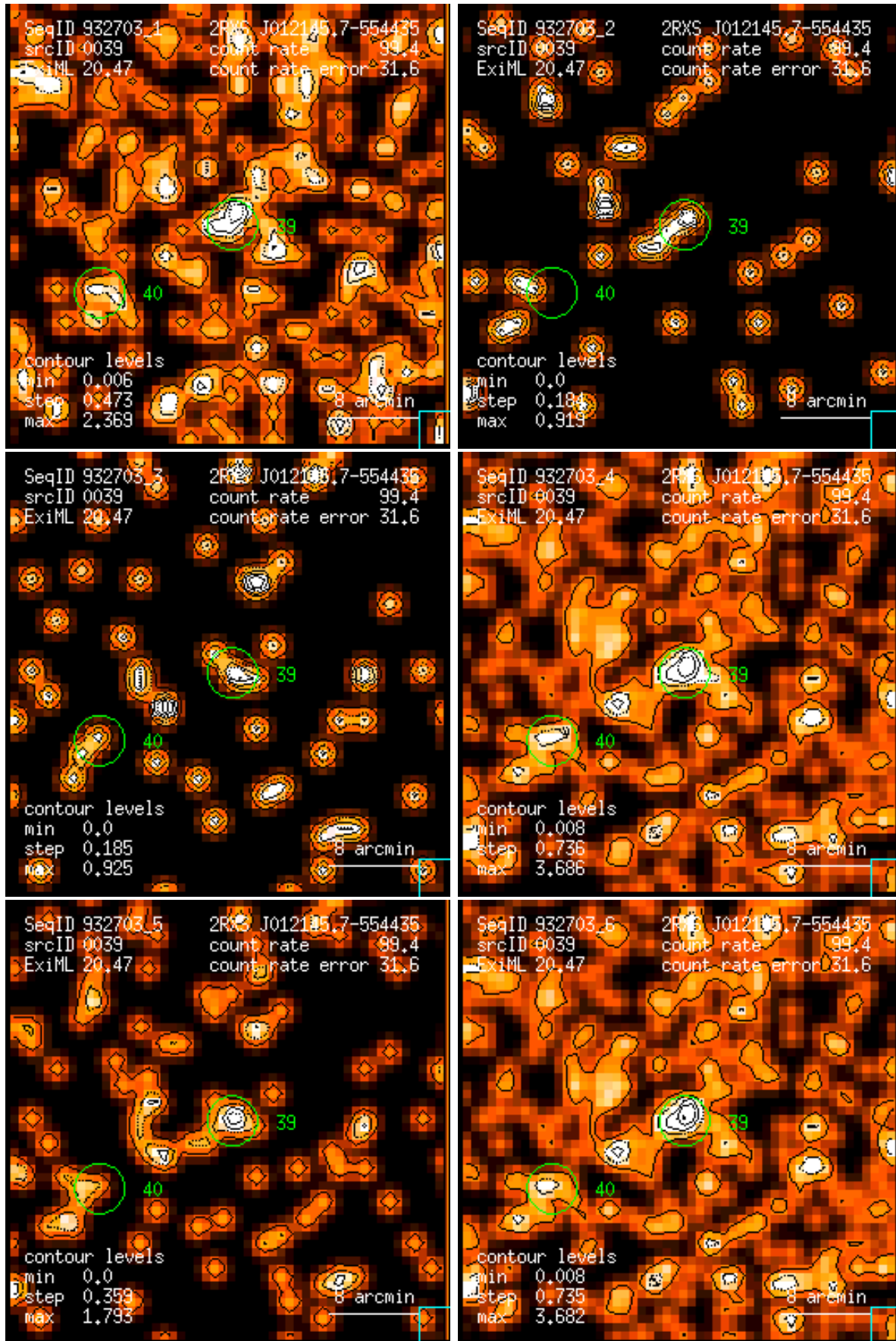
Figure 39: RASS 932703: detection 0039: band rate images, Gaussian filter: (1) PSPC channels 11 – 41, (2) 52 – 90, (3) 91 – 201, (4) 11 – 235, (5) 52 – 201, (6) 11 – 201. Broad band rates in counts/ks. Band rate contour levels in counts/ks/arcmin 2 .
