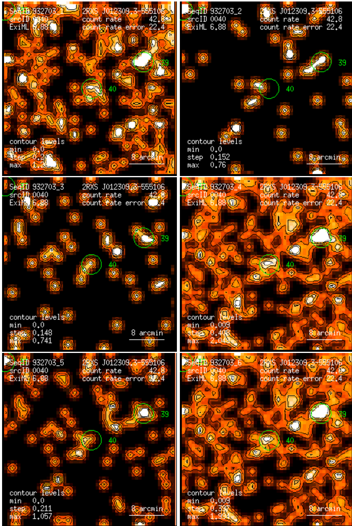
Figure 40: RASS 932703: detection 0040: band rate images, Gaussian filter: (1) PSPC channels 11 – 41, (2) 52 – 90, (3) 91 – 201, (4) 11 – 235, (5) 52 – 201, (6) 11 – 201. Broad band rates in counts/ks. Band rate contour levels in counts/ks/arcmin 2 .
