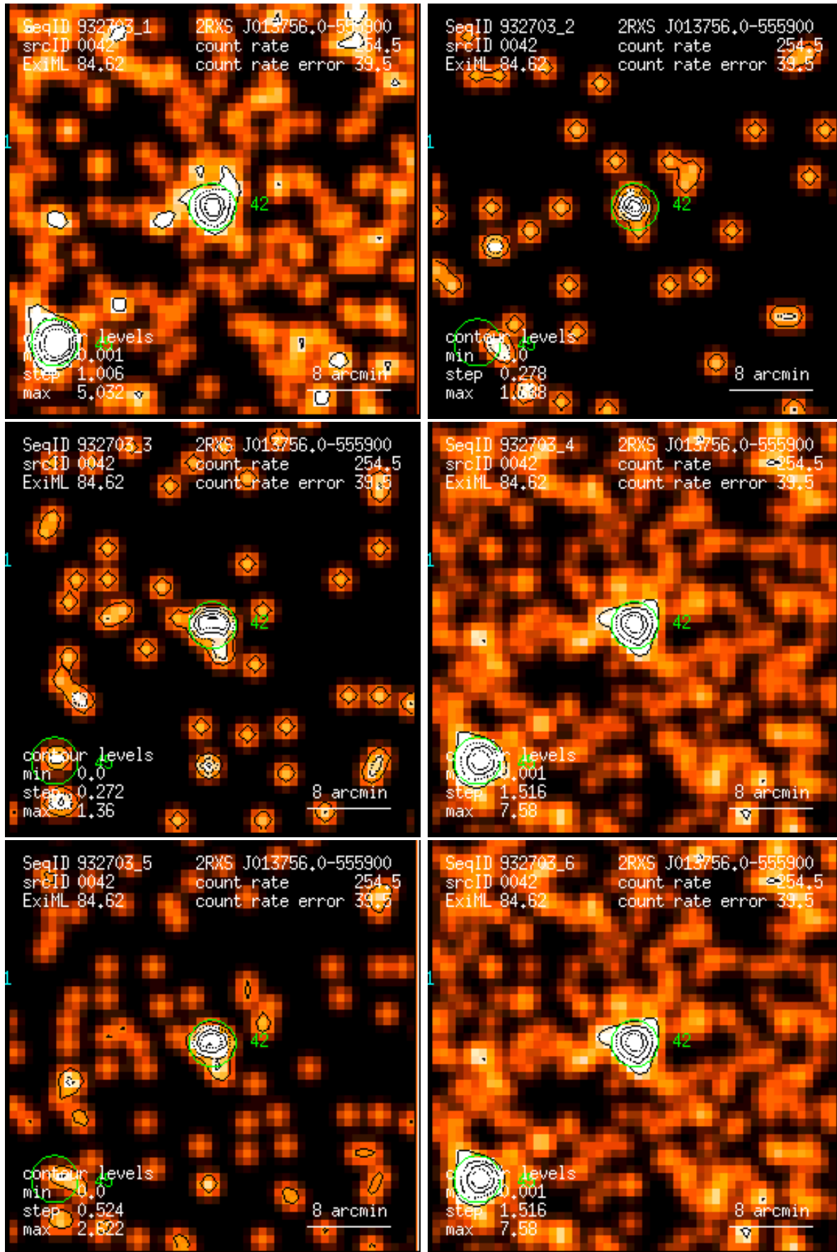
Figure 42: RASS 932703: detection 0042: band rate images, Gaussian filter: (1) PSPC channels 11 – 41, (2) 52 – 90, (3) 91 – 201, (4) 11 – 235, (5) 52 – 201, (6) 11 – 201. Broad band rates in counts/ks. Band rate contour levels in counts/ks/arcmin 2 .
