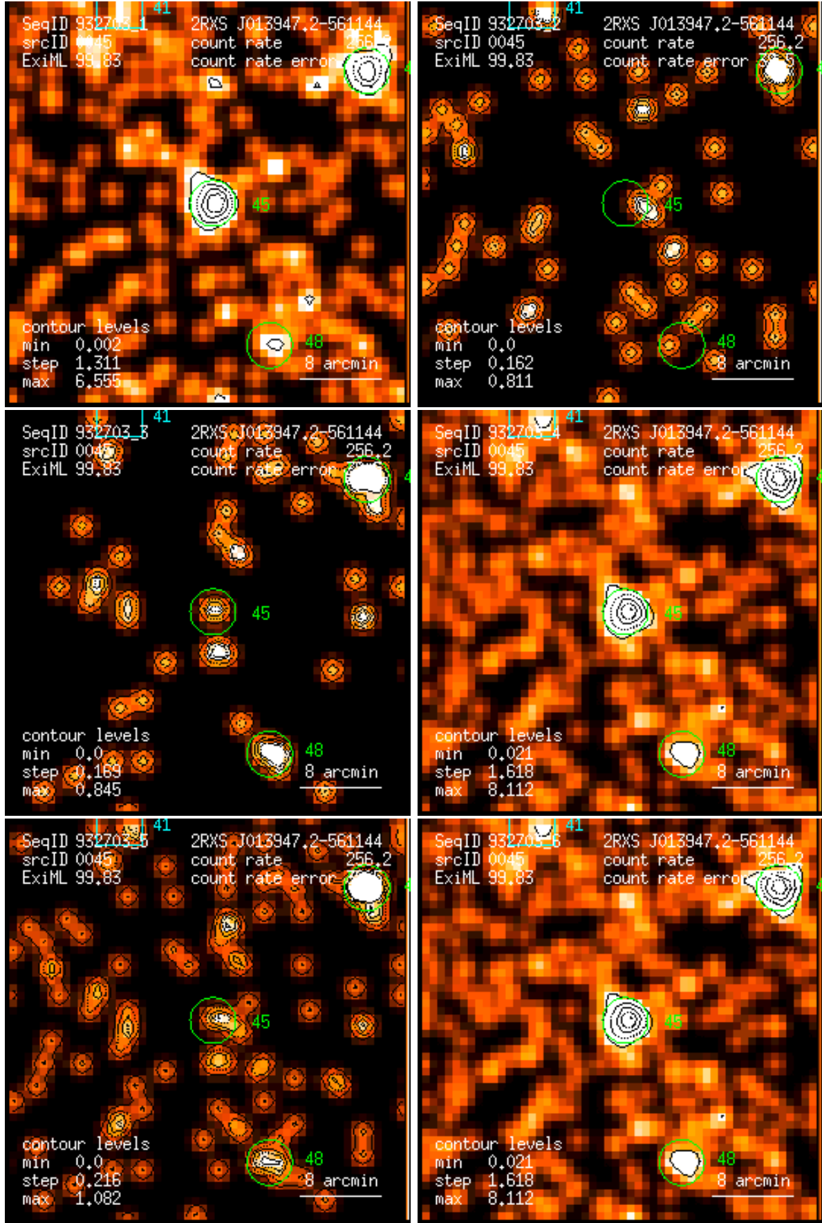
Figure 45: RASS 932703: detection 0045: band rate images, Gaussian filter: (1) PSPC channels 11 – 41, (2) 52 – 90, (3) 91 – 201, (4) 11 – 235, (5) 52 – 201, (6) 11 – 201. Broad band rates in counts/ks. Band rate contour levels in counts/ks/arcmin 2 .
