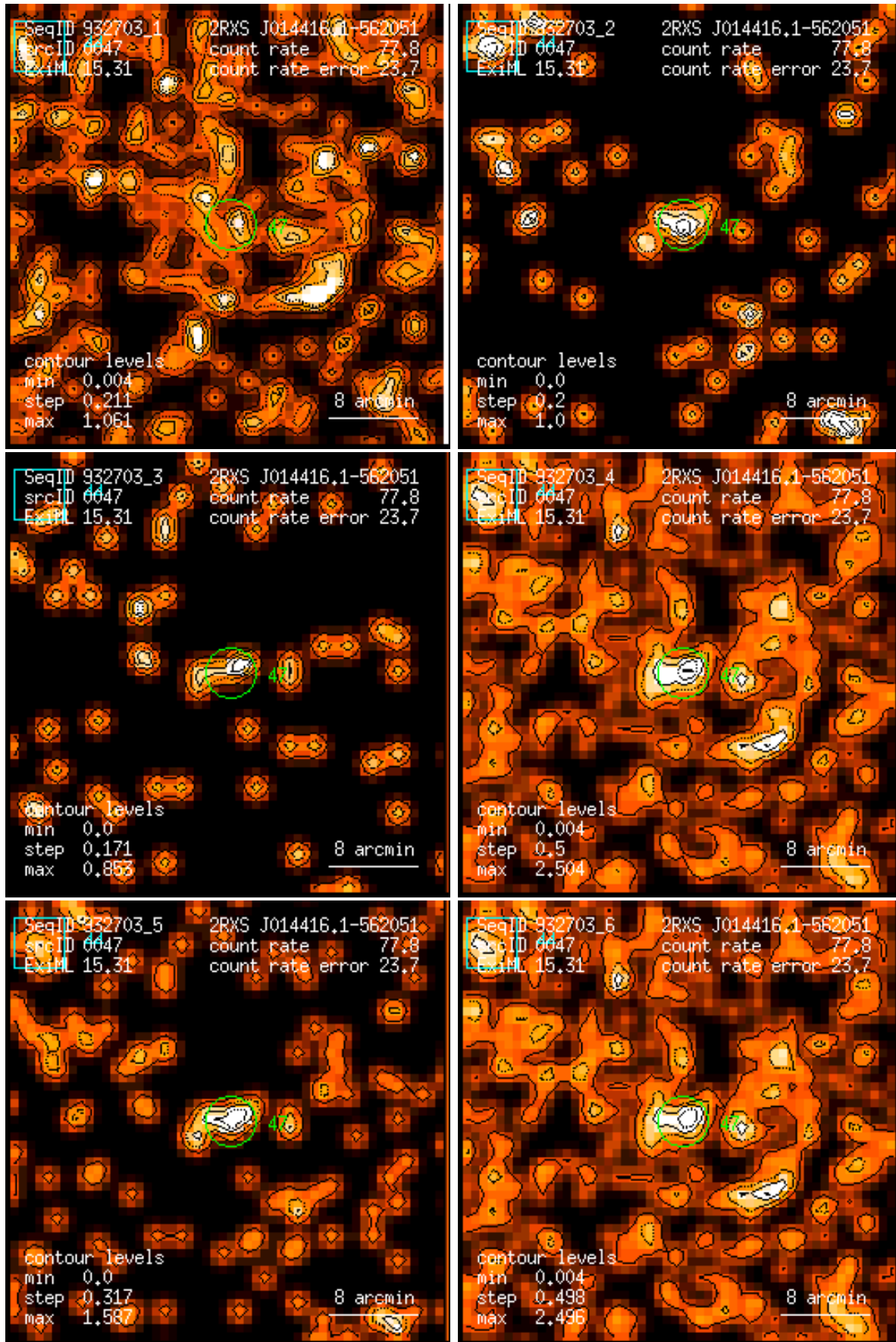
Figure 47: RASS 932703: detection 0047: band rate images, Gaussian filter: (1) PSPC channels 11 – 41, (2) 52 – 90, (3) 91 – 201, (4) 11 – 235, (5) 52 – 201, (6) 11 – 201. Broad band rates in counts/ks. Band rate contour levels in counts/ks/arcmin 2 .
