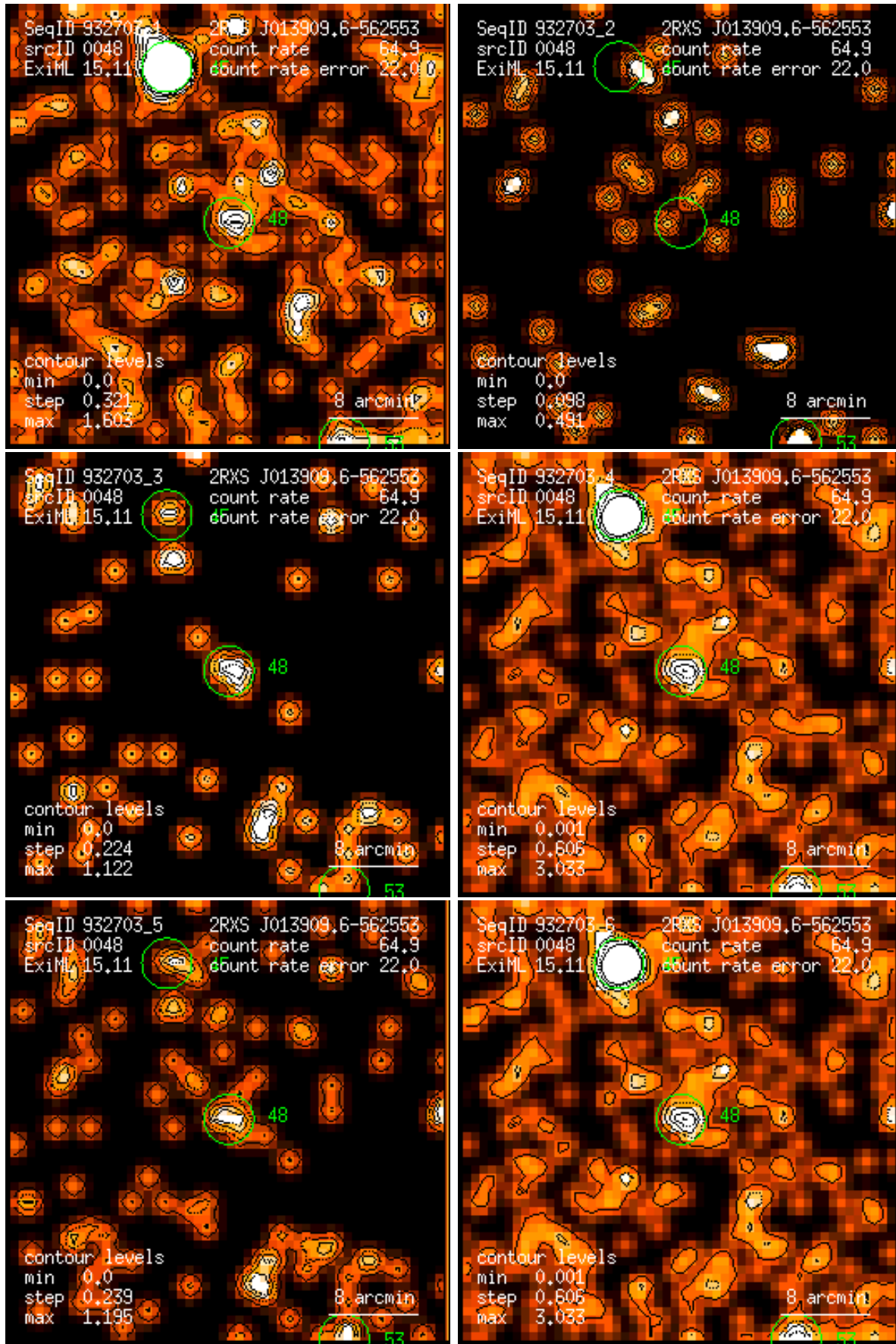
Figure 48: RASS 932703: detection 0048: band rate images, Gaussian filter: (1) PSPC channels 11 – 41, (2) 52 – 90, (3) 91 – 201, (4) 11 – 235, (5) 52 – 201, (6) 11 – 201. Broad band rates in counts/ks. Band rate contour levels in counts/ks/arcmin 2 .
