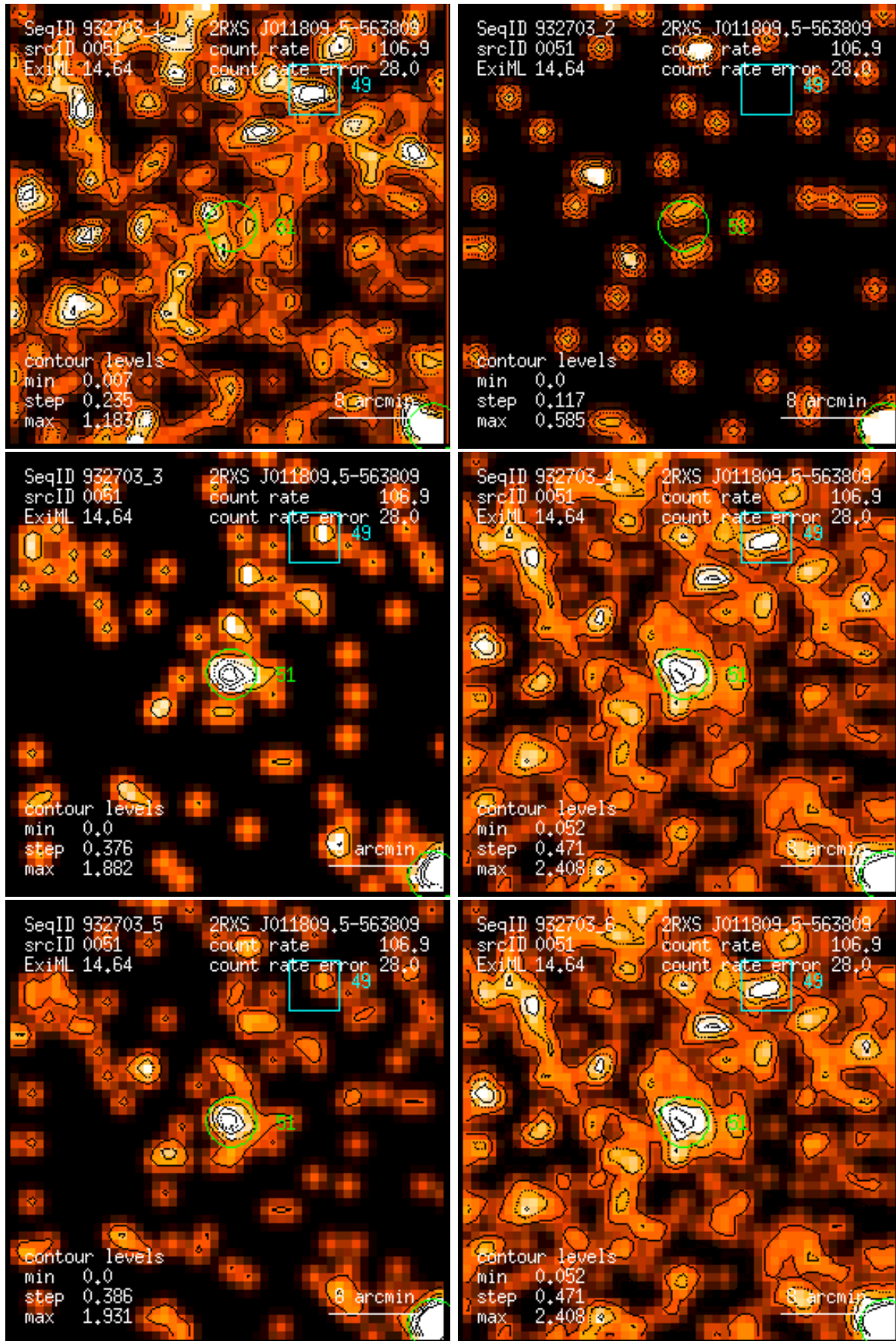
Figure 51: RASS 932703: detection 0051: band rate images, Gaussian filter: (1) PSPC channels 11 – 41, (2) 52 – 90, (3) 91 – 201, (4) 11 – 235, (5) 52 – 201, (6) 11 – 201. Broad band rates in counts/ks. Band rate contour levels in counts/ks/arcmin 2 .
