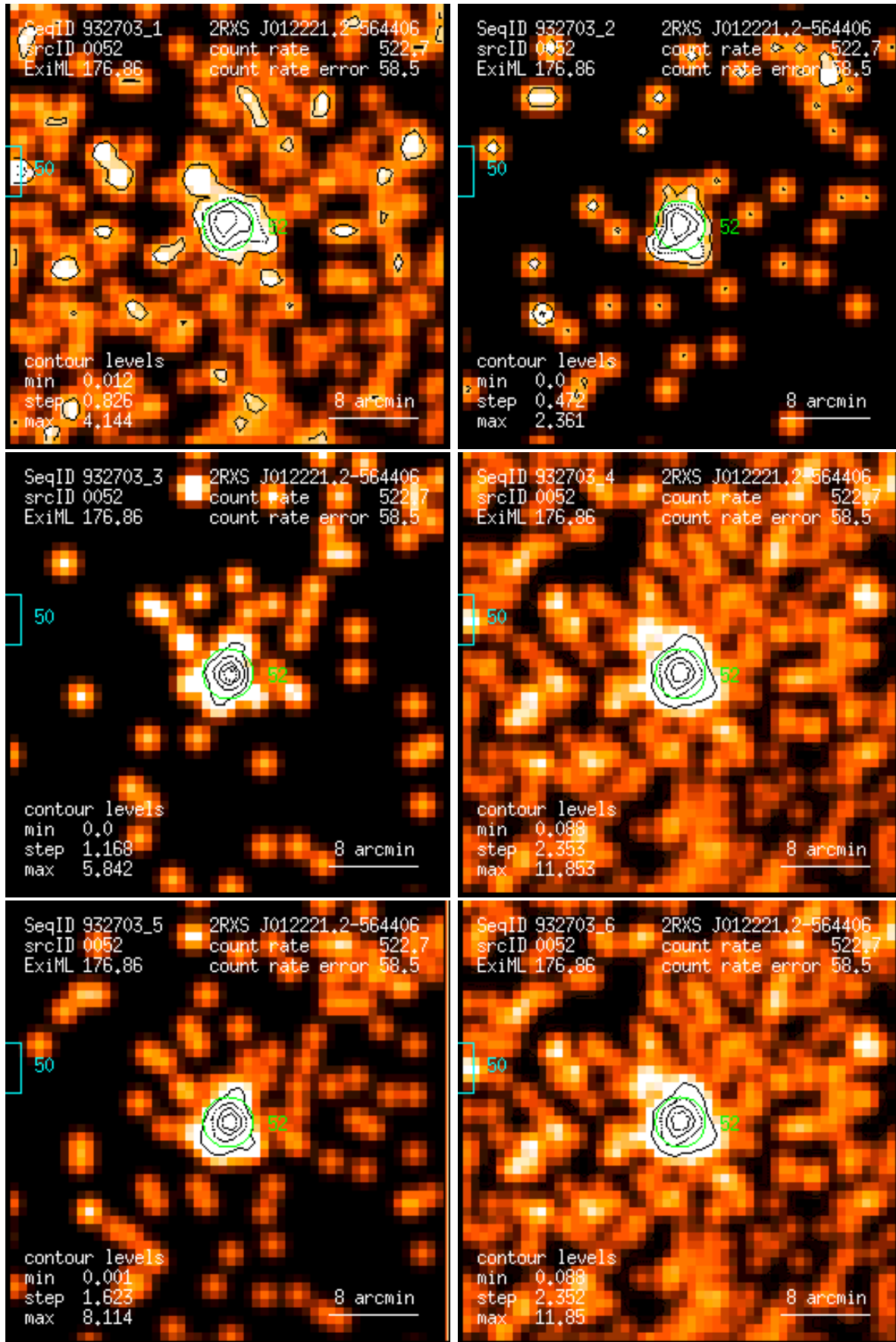
Figure 52: RASS 932703: detection 0052: band rate images, Gaussian filter: (1) PSPC channels 11 – 41, (2) 52 – 90, (3) 91 – 201, (4) 11 – 235, (5) 52 – 201, (6) 11 – 201. Broad band rates in counts/ks. Band rate contour levels in counts/ks/arcmin 2 .
