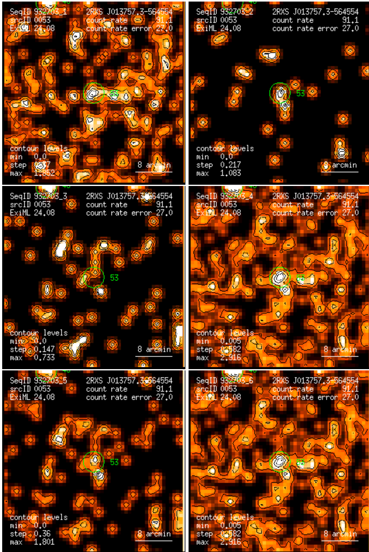
Figure 53: RASS 932703: detection 0053: band rate images, Gaussian filter: (1) PSPC channels 11 – 41, (2) 52 – 90, (3) 91 – 201, (4) 11 – 235, (5) 52 – 201, (6) 11 – 201. Broad band rates in counts/ks. Band rate contour levels in counts/ks/arcmin 2 .
