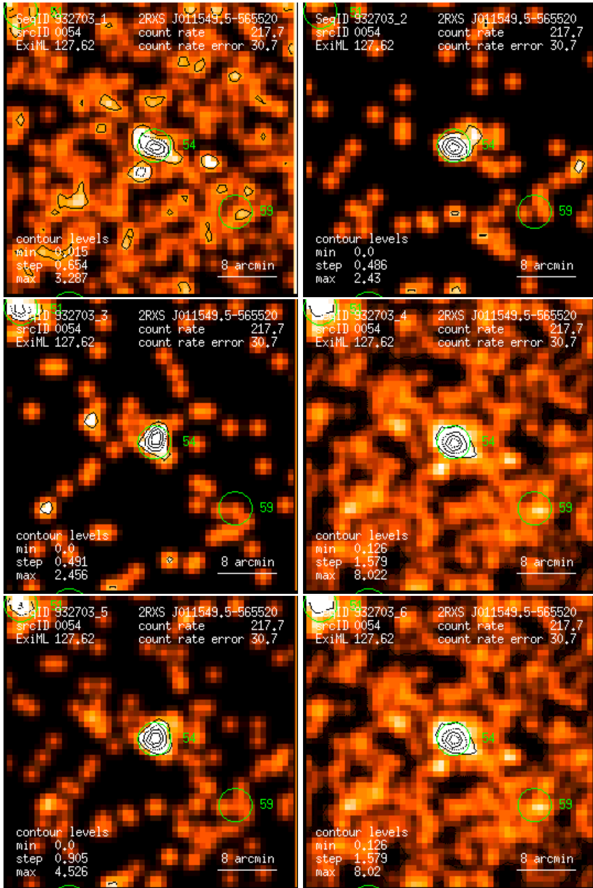
Figure 54: RASS 932703: detection 0054: band rate images, Gaussian filter: (1) PSPC channels 11 – 41, (2) 52 – 90, (3) 91 – 201, (4) 11 – 235, (5) 52 – 201, (6) 11 – 201. Broad band rates in counts/ks. Band rate contour levels in counts/ks/arcmin 2 .
