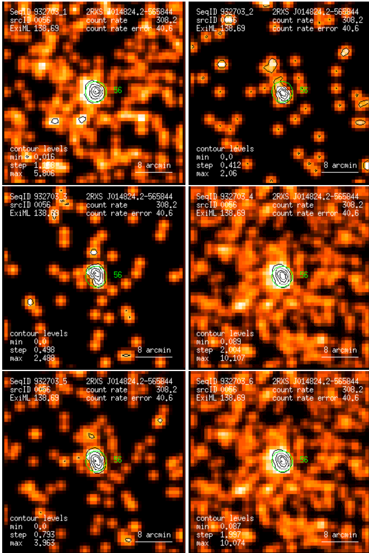
Figure 56: RASS 932703: detection 0056: band rate images, Gaussian filter: (1) PSPC channels 11 – 41, (2) 52 – 90, (3) 91 – 201, (4) 11 – 235, (5) 52 – 201, (6) 11 – 201. Broad band rates in counts/ks. Band rate contour levels in counts/ks/arcmin 2 .
