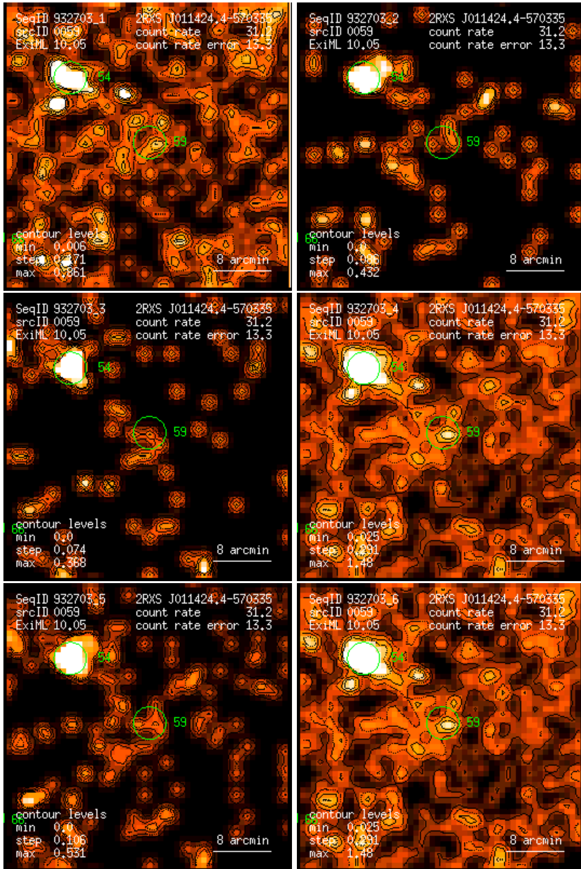
Figure 59: RASS 932703: detection 0059: band rate images, Gaussian filter: (1) PSPC channels 11 – 41, (2) 52 – 90, (3) 91 – 201, (4) 11 – 235, (5) 52 – 201, (6) 11 – 201. Broad band rates in counts/ks. Band rate contour levels in counts/ks/arcmin 2 .
