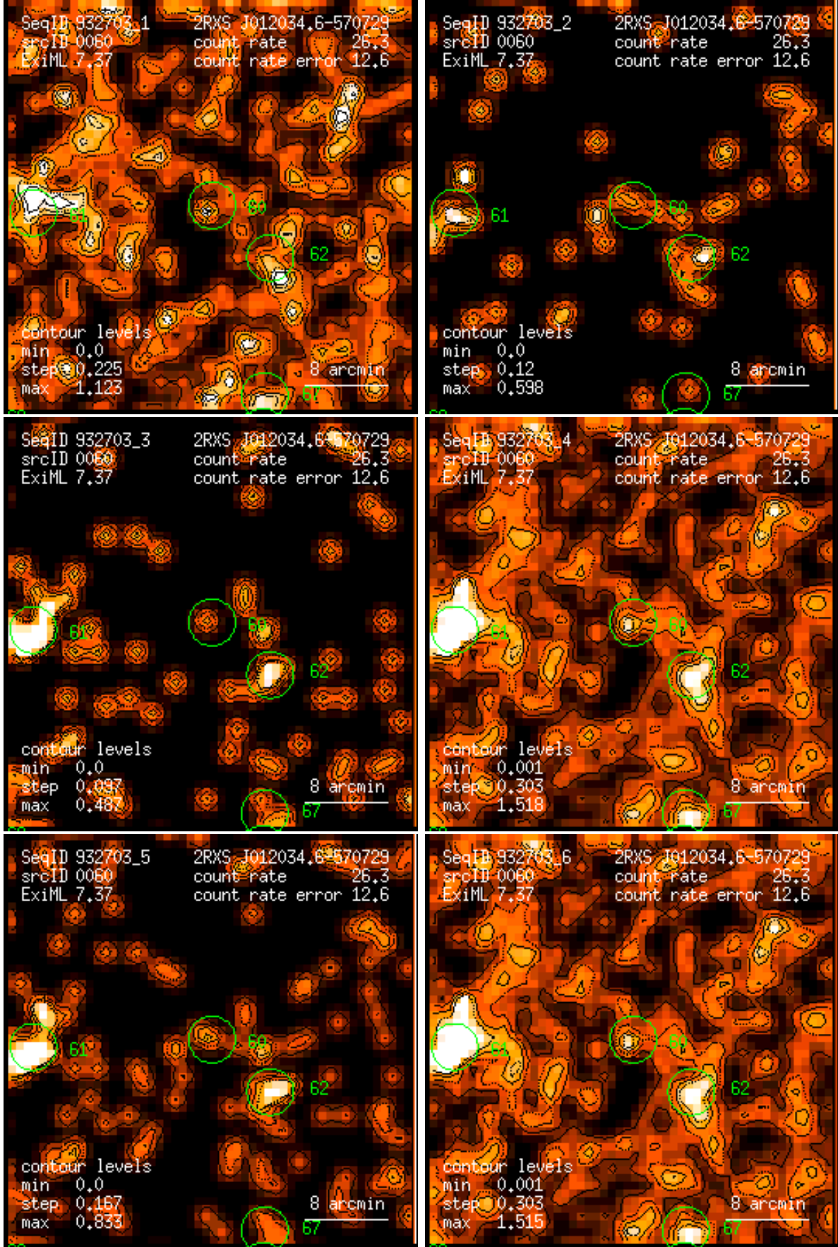
Figure 60: RASS 932703: detection 0060: band rate images, Gaussian filter: (1) PSPC channels 11 – 41, (2) 52 – 90, (3) 91 – 201, (4) 11 – 235, (5) 52 – 201, (6) 11 – 201. Broad band rates in counts/ks. Band rate contour levels in counts/ks/arcmin 2 .
