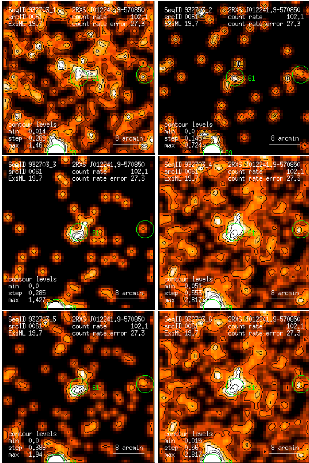
Figure 61: RASS 932703: detection 0061: band rate images, Gaussian filter: (1) PSPC channels 11 – 41, (2) 52 – 90, (3) 91 – 201, (4) 11 – 235, (5) 52 – 201, (6) 11 – 201. Broad band rates in counts/ks. Band rate contour levels in counts/ks/arcmin 2 .
