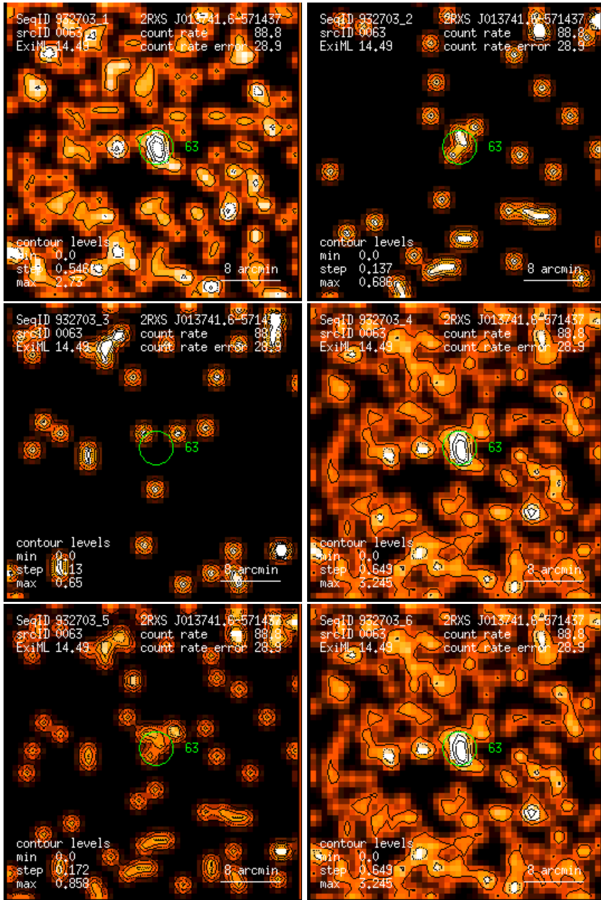
Figure 63: RASS 932703: detection 0063: band rate images, Gaussian filter: (1) PSPC channels 11 – 41, (2) 52 – 90, (3) 91 – 201, (4) 11 – 235, (5) 52 – 201, (6) 11 – 201. Broad band rates in counts/ks. Band rate contour levels in counts/ks/arcmin 2 .
