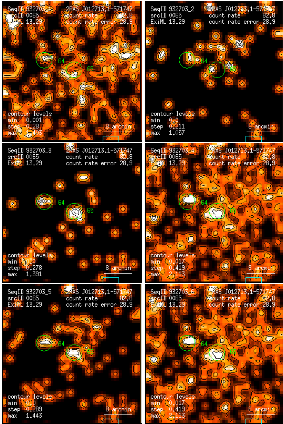
Figure 65: RASS 932703: detection 0065: band rate images, Gaussian filter: (1) PSPC channels 11 – 41, (2) 52 – 90, (3) 91 – 201, (4) 11 – 235, (5) 52 – 201, (6) 11 – 201. Broad band rates in counts/ks. Band rate contour levels in counts/ks/arcmin 2 .
