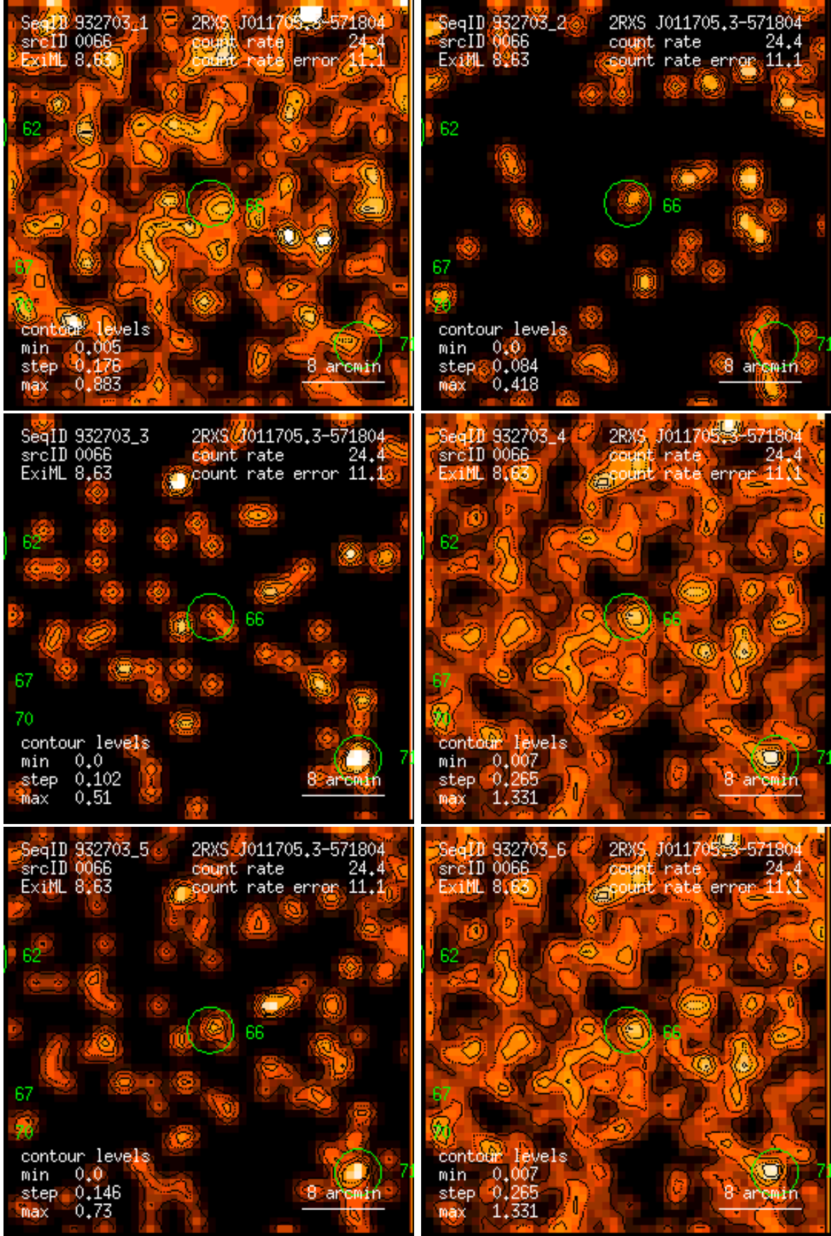
Figure 66: RASS 932703: detection 0066: band rate images, Gaussian filter: (1) PSPC channels 11 – 41, (2) 52 – 90, (3) 91 – 201, (4) 11 – 235, (5) 52 – 201, (6) 11 – 201. Broad band rates in counts/ks. Band rate contour levels in counts/ks/arcmin 2 .
