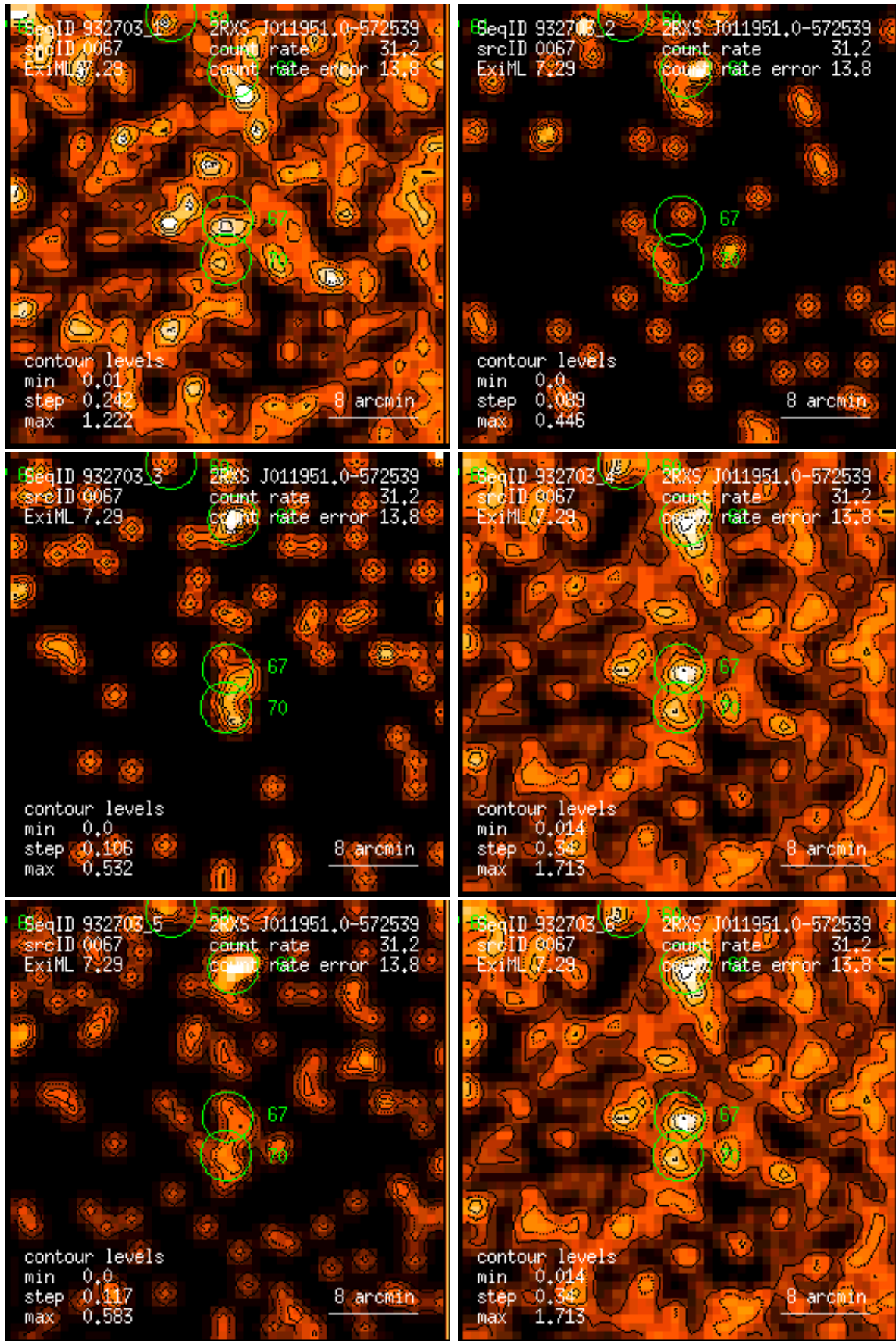
Figure 67: RASS 932703: detection 0067: band rate images, Gaussian filter: (1) PSPC channels 11 – 41, (2) 52 – 90, (3) 91 – 201, (4) 11 – 235, (5) 52 – 201, (6) 11 – 201. Broad band rates in counts/ks. Band rate contour levels in counts/ks/arcmin 2 .
