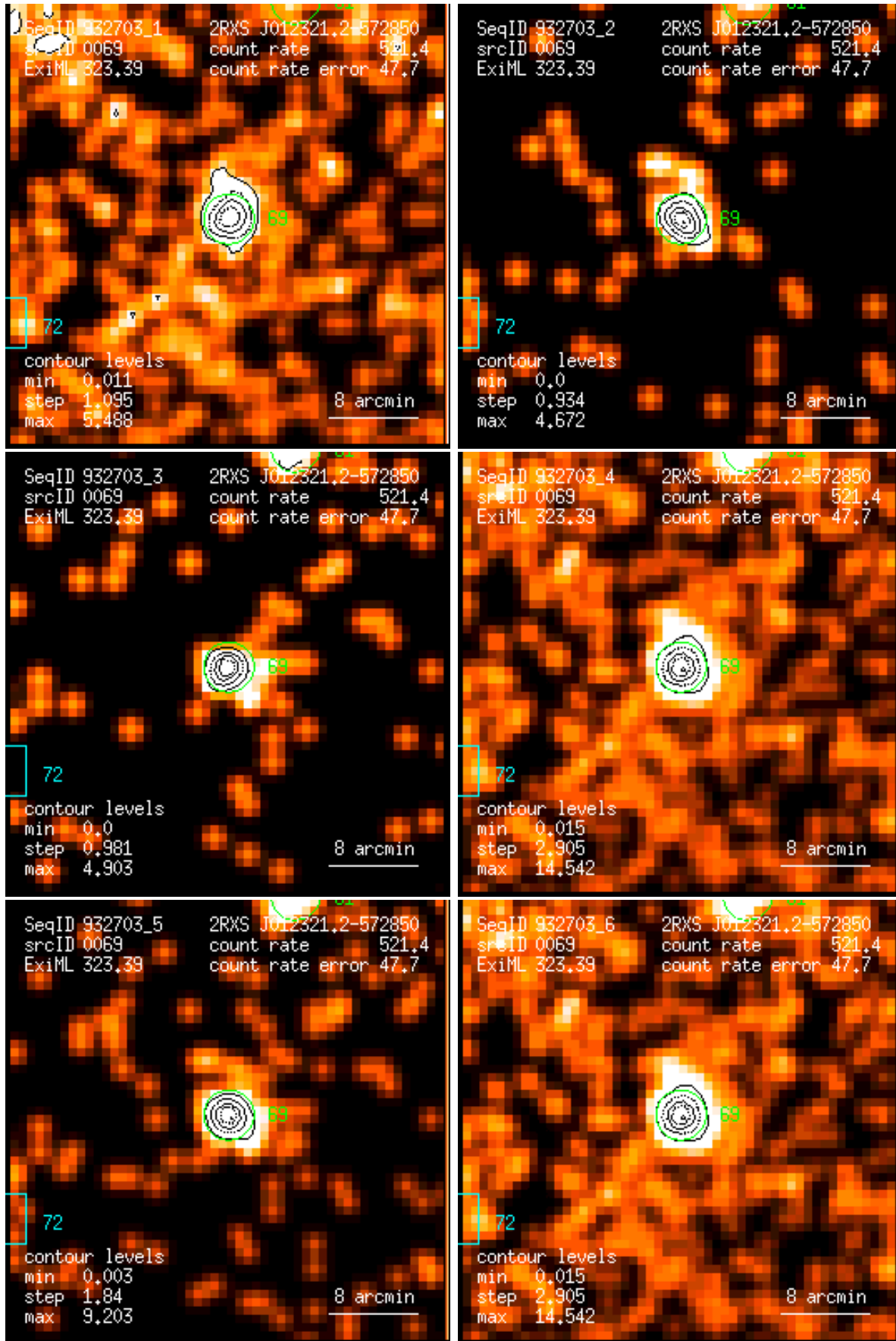
Figure 69: RASS 932703: detection 0069: band rate images, Gaussian filter: (1) PSPC channels 11 – 41, (2) 52 – 90, (3) 91 – 201, (4) 11 – 235, (5) 52 – 201, (6) 11 – 201. Broad band rates in counts/ks. Band rate contour levels in counts/ks/arcmin 2 .
