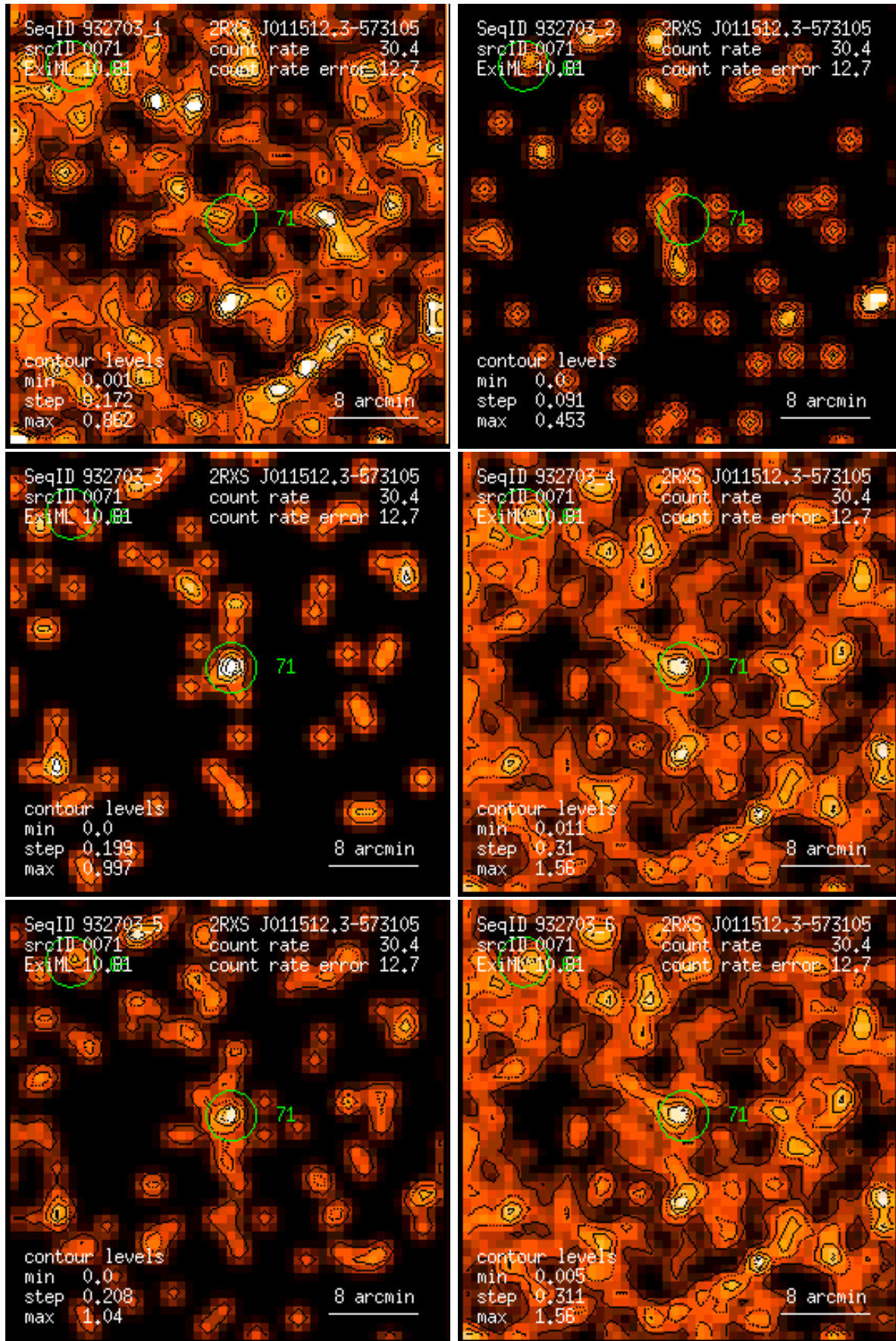
Figure 71: RASS 932703: detection 0071: band rate images, Gaussian filter: (1) PSPC channels 11 – 41, (2) 52 – 90, (3) 91 – 201, (4) 11 – 235, (5) 52 – 201, (6) 11 – 201. Broad band rates in counts/ks. Band rate contour levels in counts/ks/arcmin 2 .
