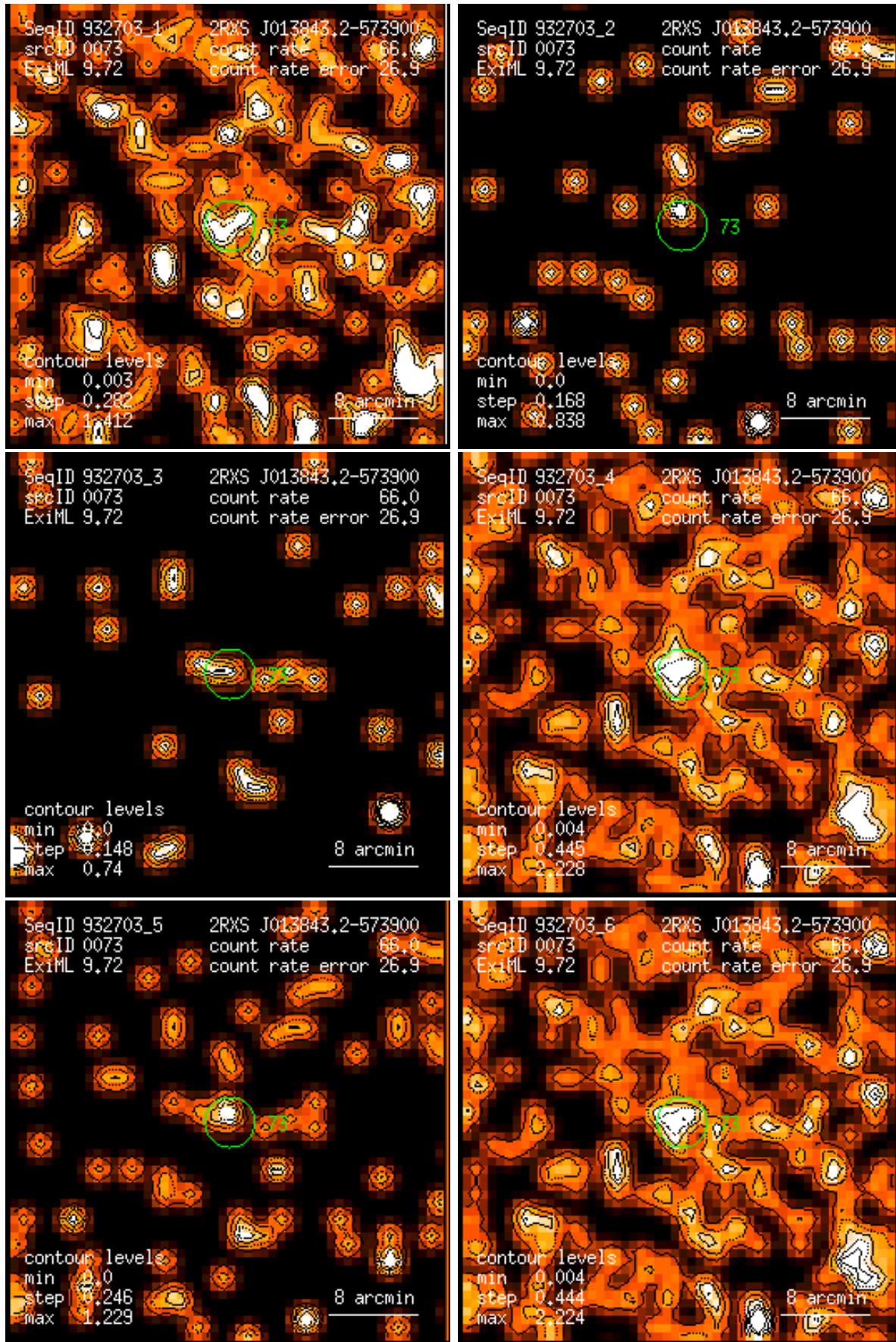
Figure 73: RASS 932703: detection 0073: band rate images, Gaussian filter: (1) PSPC channels 11 – 41, (2) 52 – 90, (3) 91 – 201, (4) 11 – 235, (5) 52 – 201, (6) 11 – 201. Broad band rates in counts/ks. Band rate contour levels in counts/ks/arcmin 2 .
