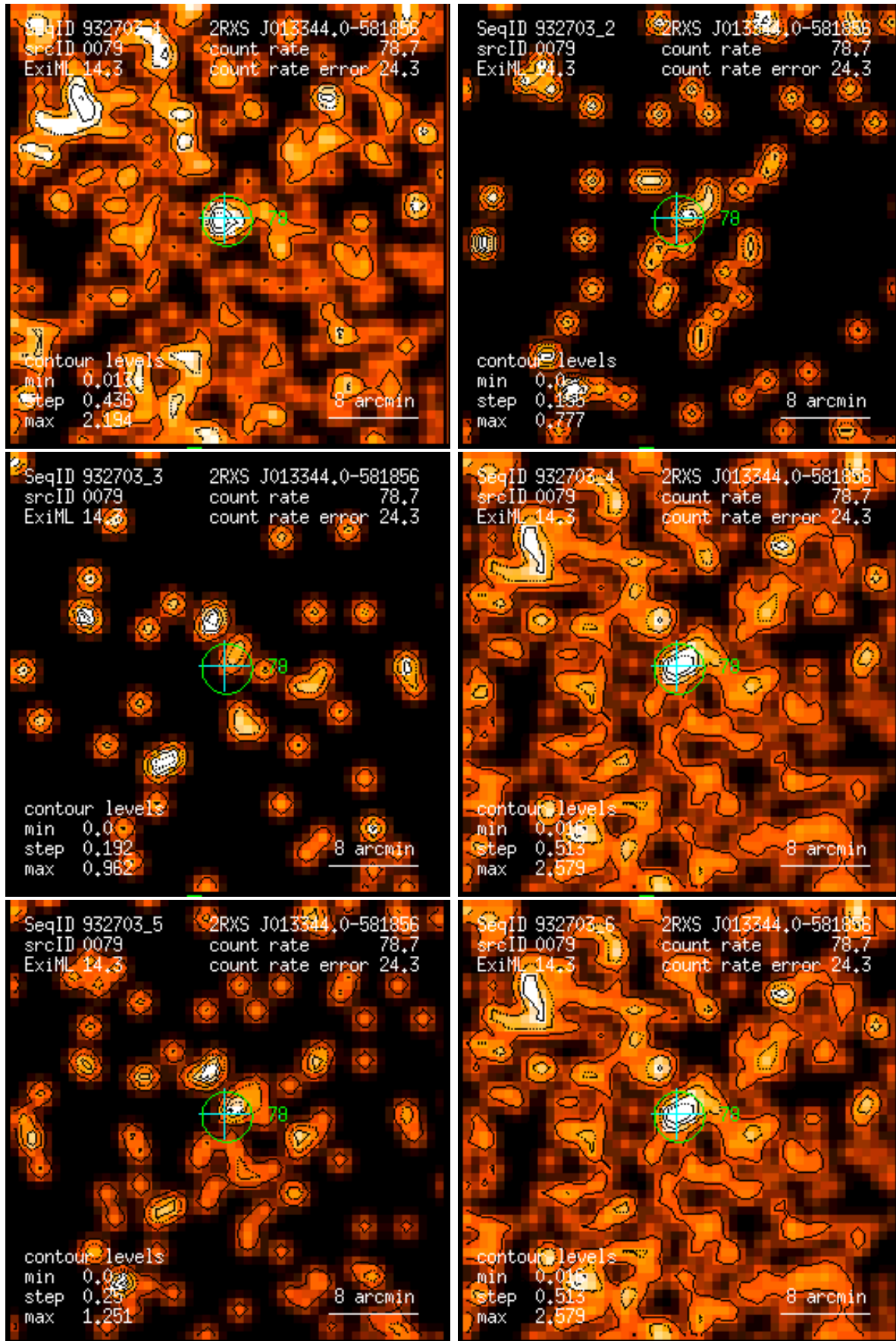
Figure 79: RASS 932703: detection 0079: band rate images, Gaussian filter: (1) PSPC channels 11 – 41, (2) 52 – 90, (3) 91 – 201, (4) 11 – 235, (5) 52 – 201, (6) 11 – 201. Broad band rates in counts/ks. Band rate contour levels in counts/ks/arcmin 2 .
