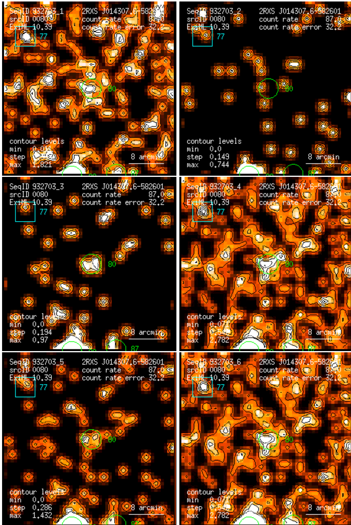
Figure 80: RASS 932703: detection 0080: band rate images, Gaussian filter: (1) PSPC channels 11 – 41, (2) 52 – 90, (3) 91 – 201, (4) 11 – 235, (5) 52 – 201, (6) 11 – 201. Broad band rates in counts/ks. Band rate contour levels in counts/ks/arcmin 2 .
