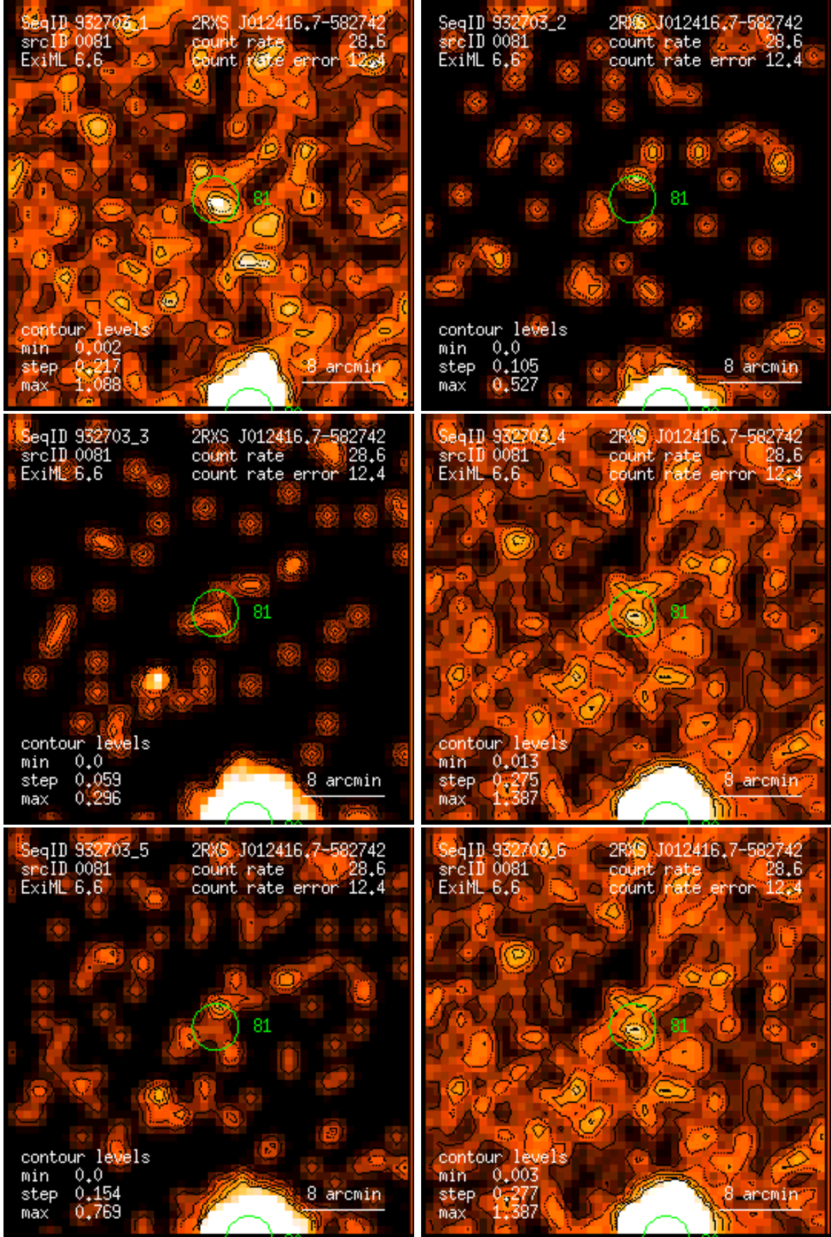
Figure 81: RASS 932703: detection 0081: band rate images, Gaussian filter: (1) PSPC channels 11 – 41, (2) 52 – 90, (3) 91 – 201, (4) 11 – 235, (5) 52 – 201, (6) 11 – 201. Broad band rates in counts/ks. Band rate contour levels in counts/ks/arcmin 2 .
