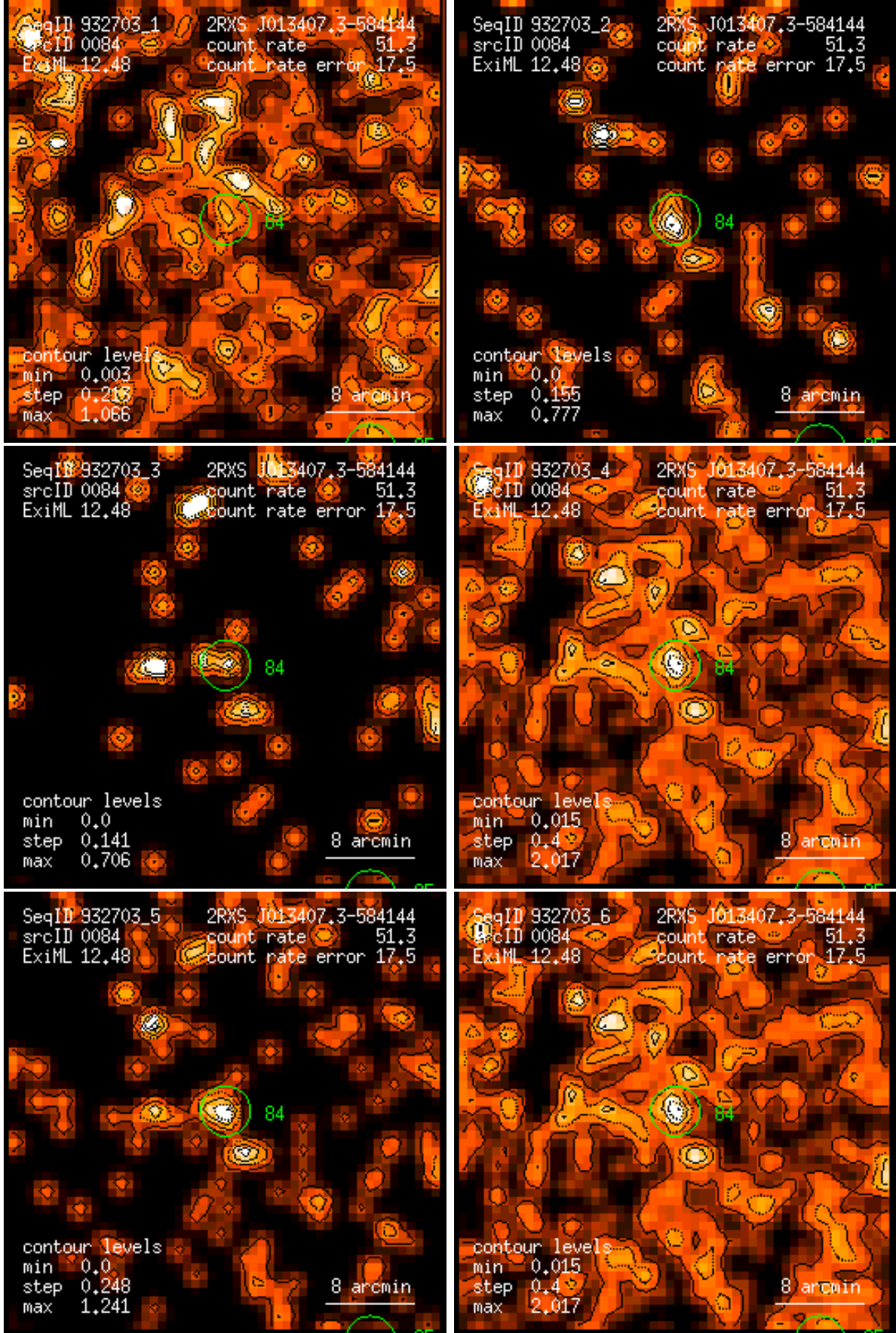
Figure 84: RASS 932703: detection 0084: band rate images, Gaussian filter: (1) PSPC channels 11 – 41, (2) 52 – 90, (3) 91 – 201, (4) 11 – 235, (5) 52 – 201, (6) 11 – 201. Broad band rates in counts/ks. Band rate contour levels in counts/ks/arcmin 2 .
