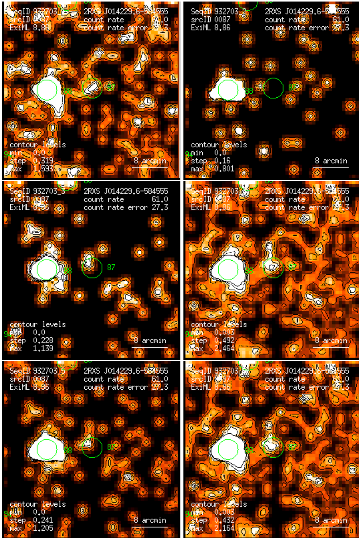
Figure 87: RASS 932703: detection 0087: band rate images, Gaussian filter: (1) PSPC channels 11 – 41, (2) 52 – 90, (3) 91 – 201, (4) 11 – 235, (5) 52 – 201, (6) 11 – 201. Broad band rates in counts/ks. Band rate contour levels in counts/ks/arcmin 2 .
