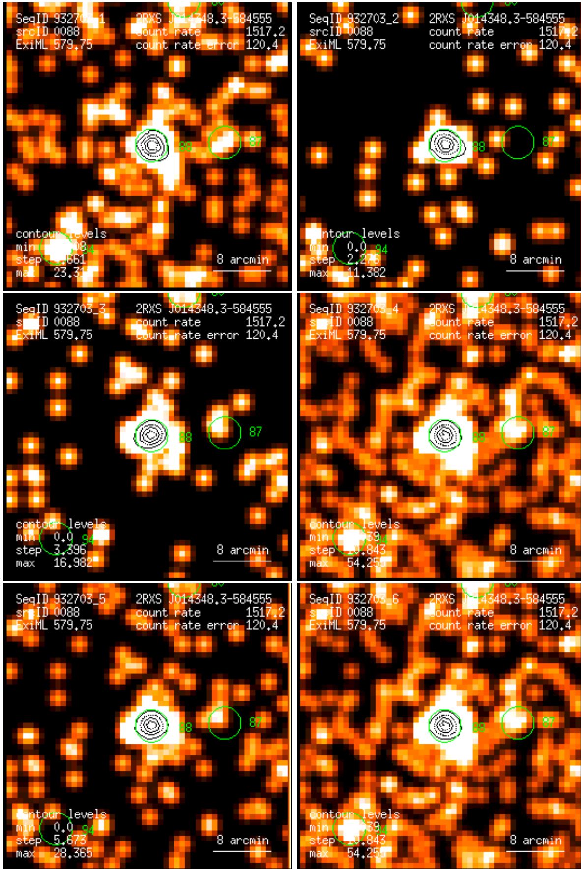
Figure 88: RASS 932703: detection 0088: band rate images, Gaussian filter: (1) PSPC channels 11 – 41, (2) 52 – 90, (3) 91 – 201, (4) 11 – 235, (5) 52 – 201, (6) 11 – 201. Broad band rates in counts/ks. Band rate contour levels in counts/ks/arcmin 2 .
