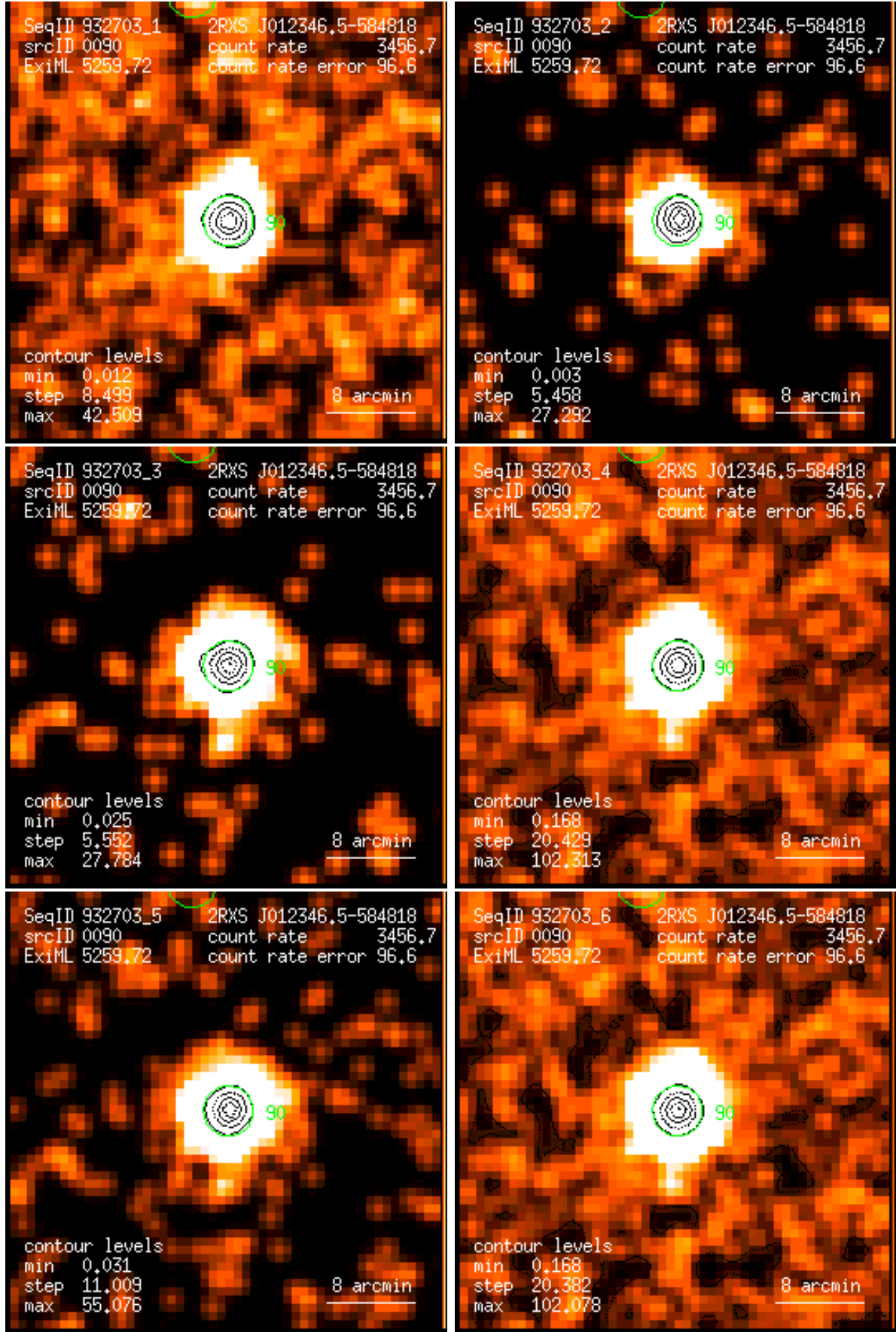
Figure 90: RASS 932703: detection 0090: band rate images, Gaussian filter: (1) PSPC channels 11 – 41, (2) 52 – 90, (3) 91 – 201, (4) 11 – 235, (5) 52 – 201, (6) 11 – 201. Broad band rates in counts/ks. Band rate contour levels in counts/ks/arcmin 2 .
