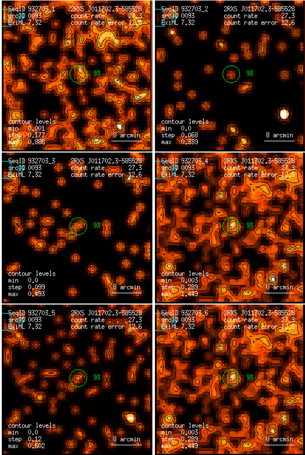
Figure 93: RASS 932703: detection 0093: band rate images, Gaussian filter: (1) PSPC channels 11 – 41, (2) 52 – 90, (3) 91 – 201, (4) 11 – 235, (5) 52 – 201, (6) 11 – 201. Broad band rates in counts/ks. Band rate contour levels in counts/ks/arcmin 2 .
