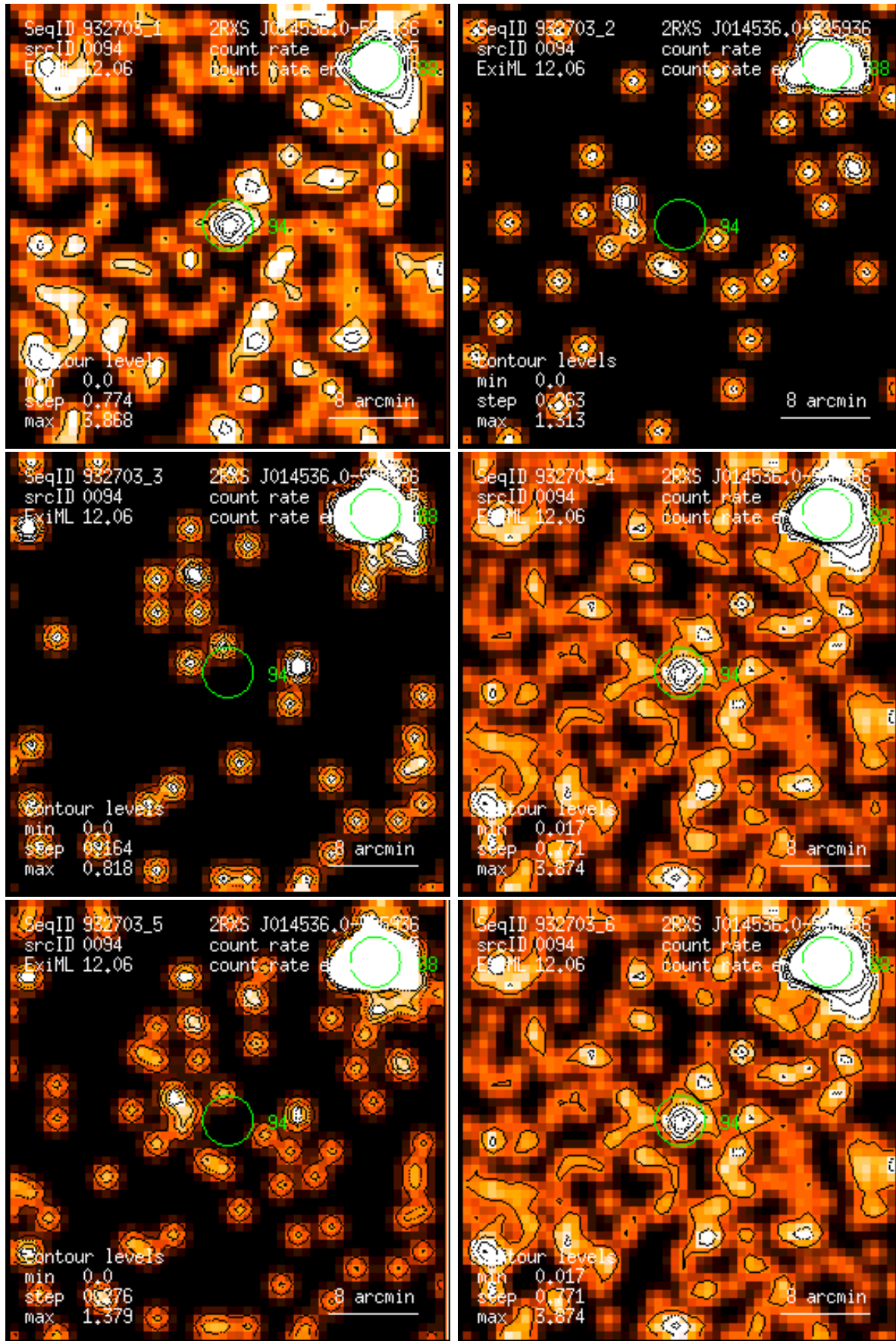
Figure 94: RASS 932703: detection 0094: band rate images, Gaussian filter: (1) PSPC channels 11 – 41, (2) 52 – 90, (3) 91 – 201, (4) 11 – 235, (5) 52 – 201, (6) 11 – 201. Broad band rates in counts/ks. Band rate contour levels in counts/ks/arcmin 2 .
