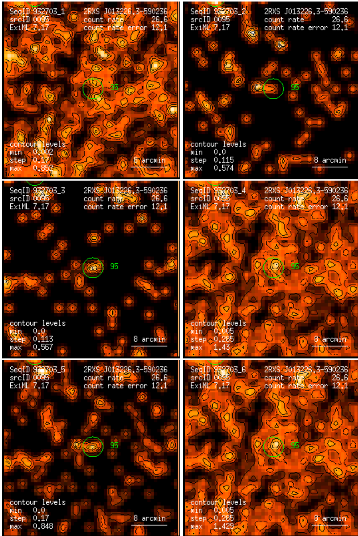
Figure 95: RASS 932703: detection 0095: band rate images, Gaussian filter: (1) PSPC channels 11 – 41, (2) 52 – 90, (3) 91 – 201, (4) 11 – 235, (5) 52 – 201, (6) 11 – 201. Broad band rates in counts/ks. Band rate contour levels in counts/ks/arcmin 2 .
