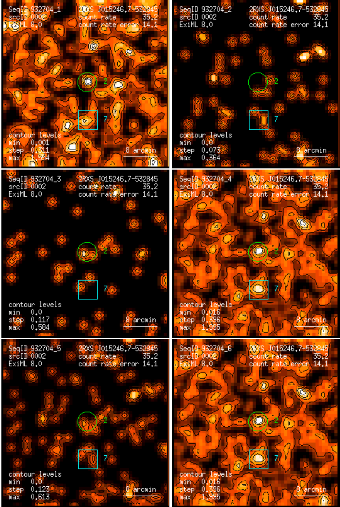
Figure 2: RASS 932704: detection 0002: band rate images, Gaussian filter: (1) PSPC channels 11 – 41, (2) 52 – 90, (3) 91 – 201, (4) 11 – 235, (5) 52 – 201, (6) 11 – 201. Broad band rates in counts/ks. Band rate contour levels in counts/ks/arcmin 2 .
