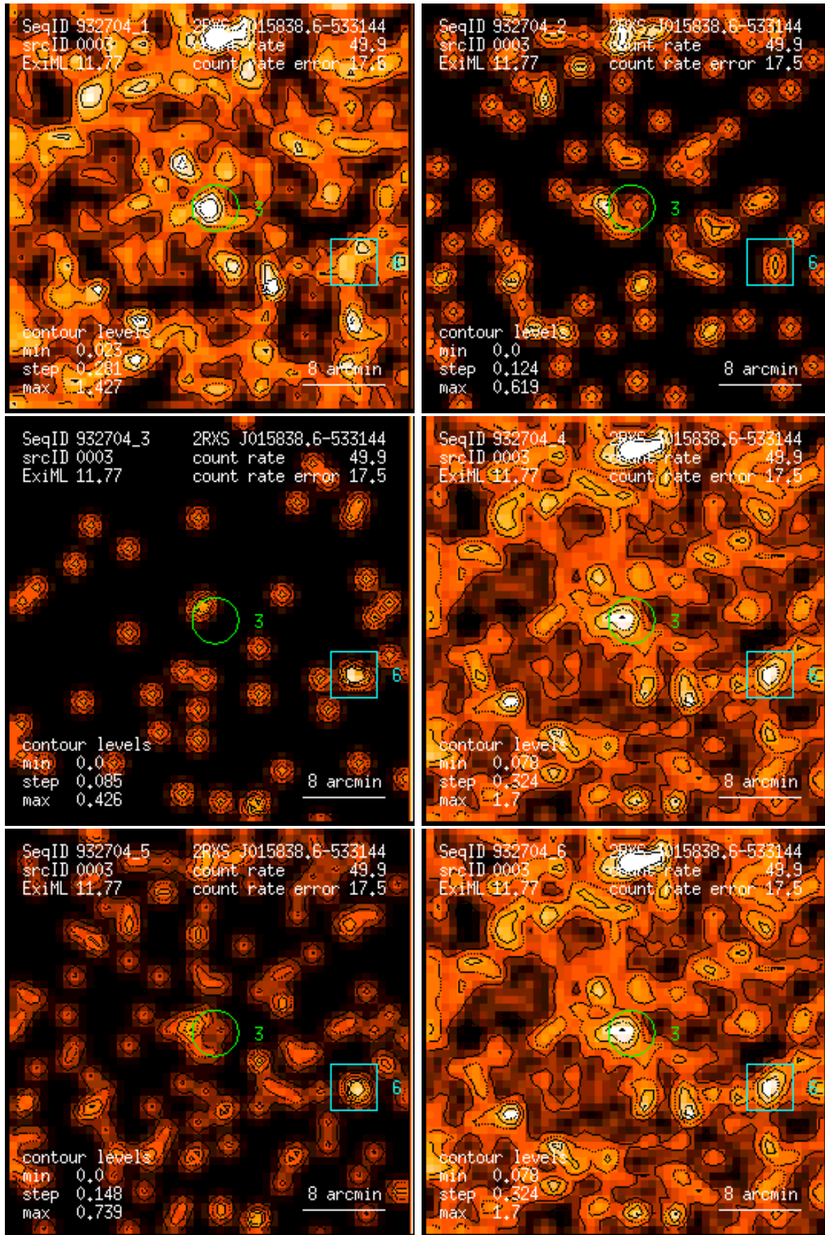
Figure 3: RASS 932704: detection 0003: band rate images, Gaussian filter: (1) PSPC channels 11 – 41, (2) 52 – 90, (3) 91 – 201, (4) 11 – 235, (5) 52 – 201, (6) 11 – 201. Broad band rates in counts/ks. Band rate contour levels in counts/ks/arcmin 2 .
