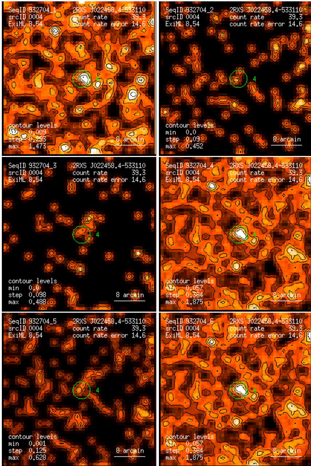
Figure 4: RASS 932704: detection 0004: band rate images, Gaussian filter: (1) PSPC channels 11 – 41, (2) 52 – 90, (3) 91 – 201, (4) 11 – 235, (5) 52 – 201, (6) 11 – 201. Broad band rates in counts/ks. Band rate contour levels in counts/ks/arcmin 2 .
