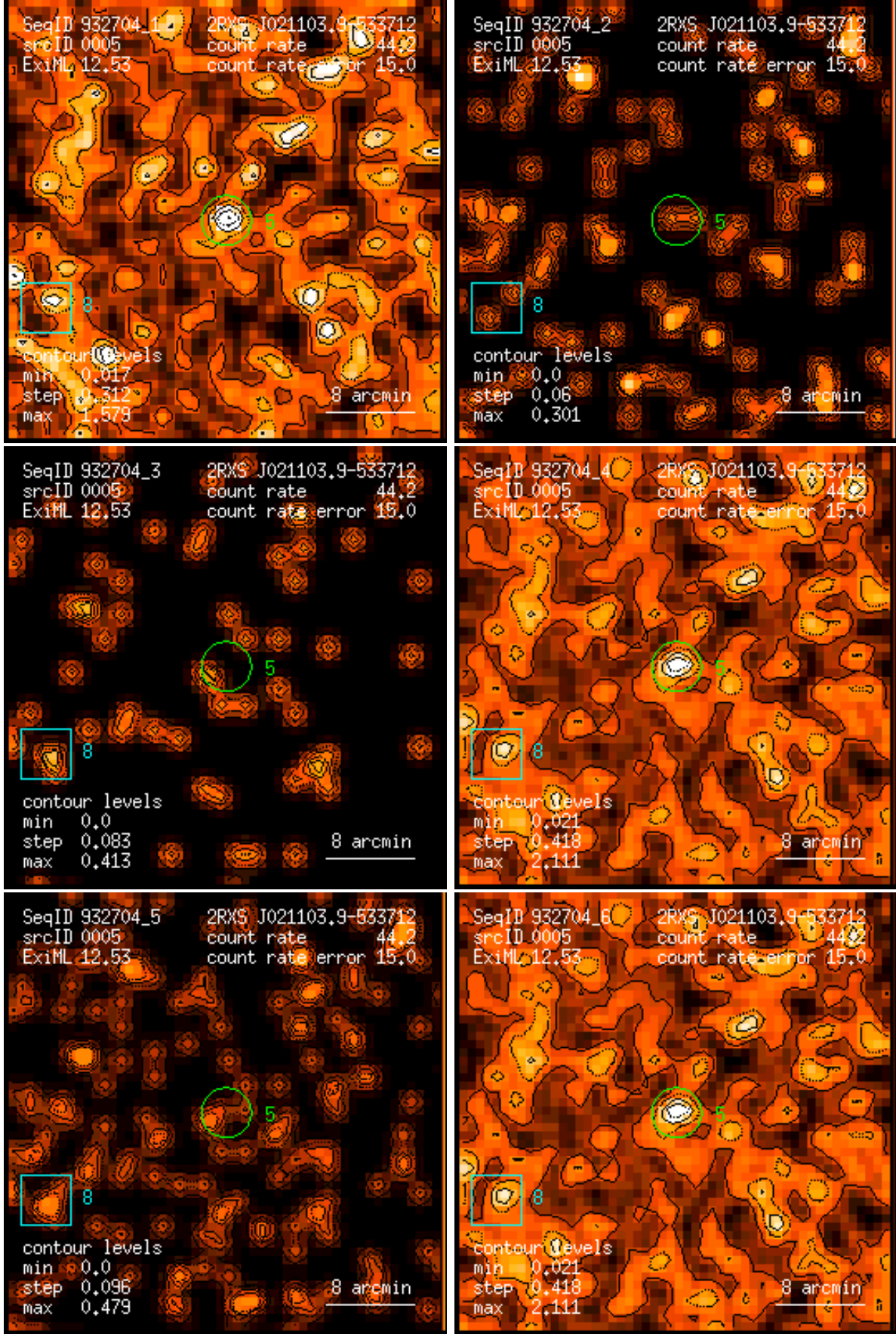
Figure 5: RASS 932704: detection 0005: band rate images, Gaussian filter: (1) PSPC channels 11 – 41, (2) 52 – 90, (3) 91 – 201, (4) 11 – 235, (5) 52 – 201, (6) 11 – 201. Broad band rates in counts/ks. Band rate contour levels in counts/ks/arcmin 2 .
