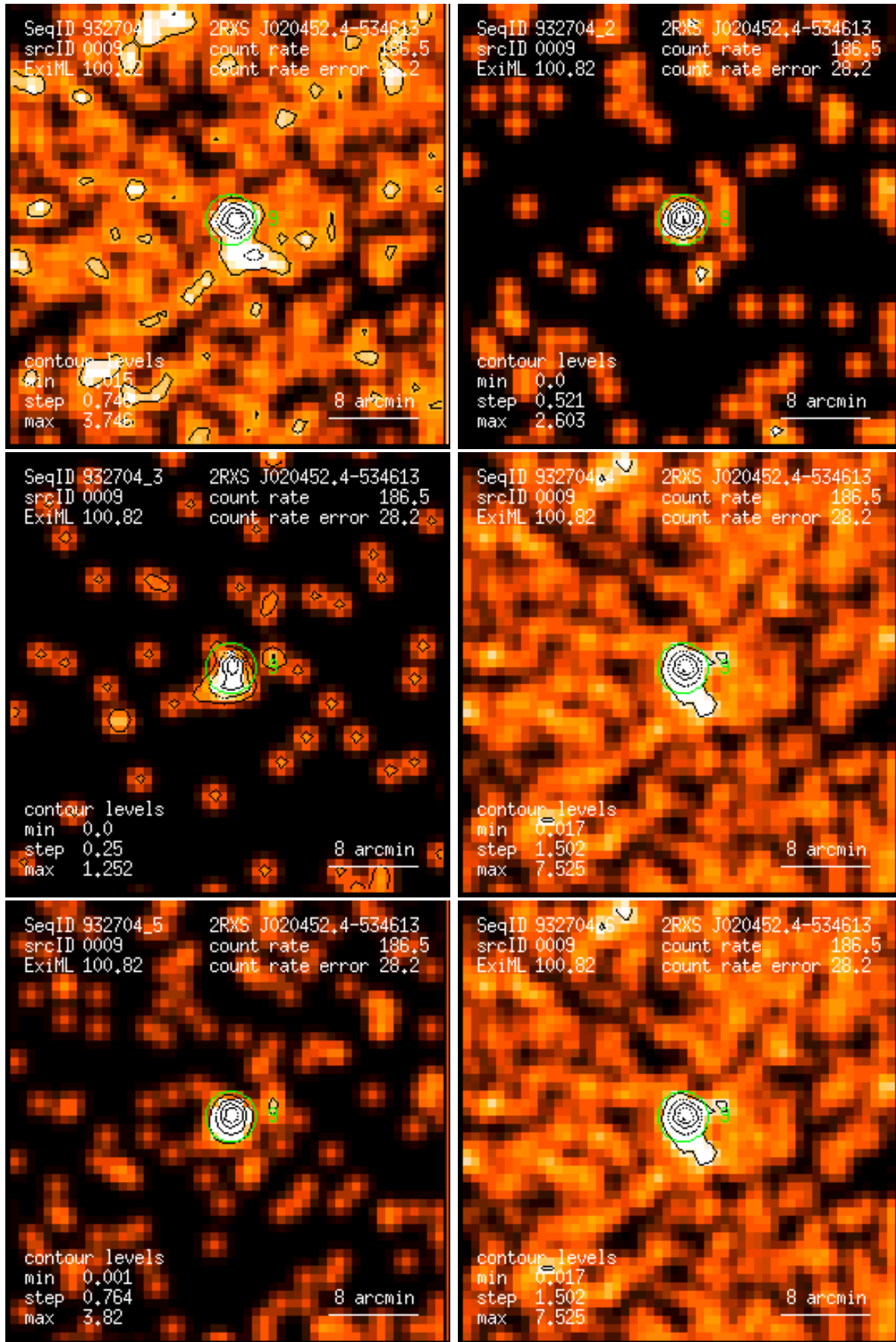
Figure 9: RASS 932704: detection 0009: band rate images, Gaussian filter: (1) PSPC channels 11 – 41, (2) 52 – 90, (3) 91 – 201, (4) 11 – 235, (5) 52 – 201, (6) 11 – 201. Broad band rates in counts/ks. Band rate contour levels in counts/ks/arcmin 2 .
