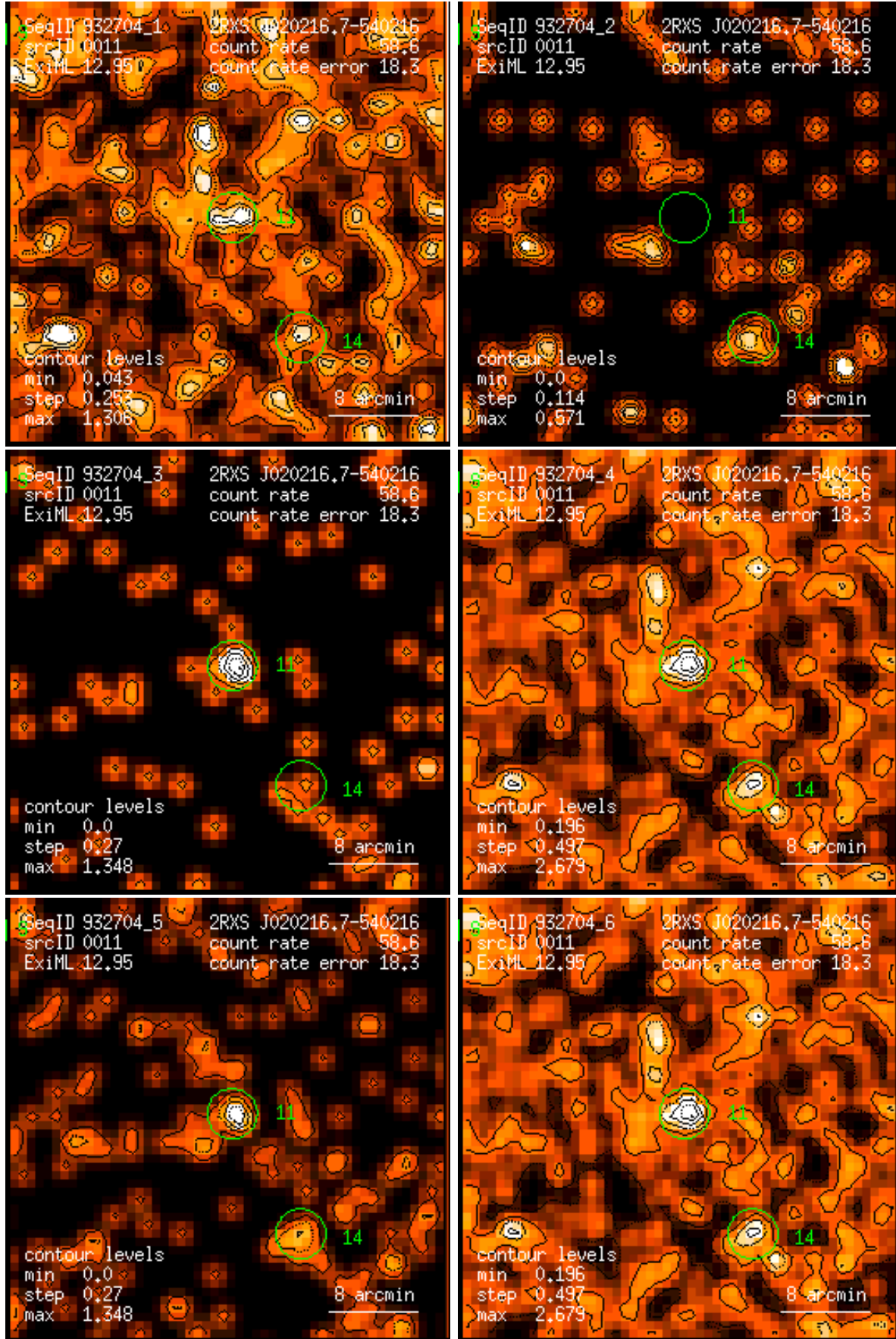
Figure 11: RASS 932704: detection 0011: band rate images, Gaussian filter: (1) PSPC channels 11 – 41, (2) 52 – 90, (3) 91 – 201, (4) 11 – 235, (5) 52 – 201, (6) 11 – 201. Broad band rates in counts/ks. Band rate contour levels in counts/ks/arcmin 2 .
