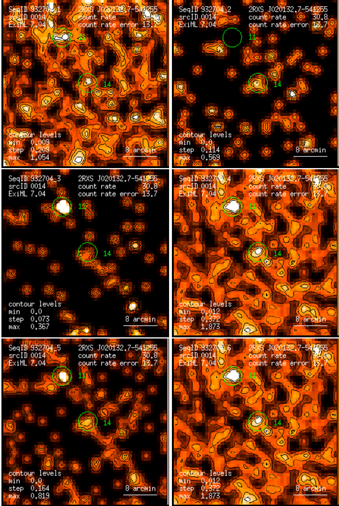
Figure 14: RASS 932704: detection 0014: band rate images, Gaussian filter: (1) PSPC channels 11 – 41, (2) 52 – 90, (3) 91 – 201, (4) 11 – 235, (5) 52 – 201, (6) 11 – 201. Broad band rates in counts/ks. Band rate contour levels in counts/ks/arcmin 2 .
