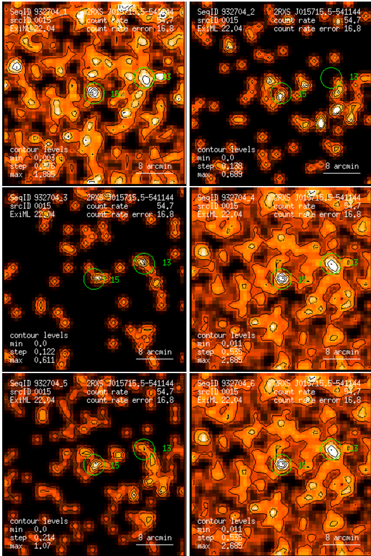
Figure 15: RASS 932704: detection 0015: band rate images, Gaussian filter: (1) PSPC channels 11 – 41, (2) 52 – 90, (3) 91 – 201, (4) 11 – 235, (5) 52 – 201, (6) 11 – 201. Broad band rates in counts/ks. Band rate contour levels in counts/ks/arcmin 2 .
