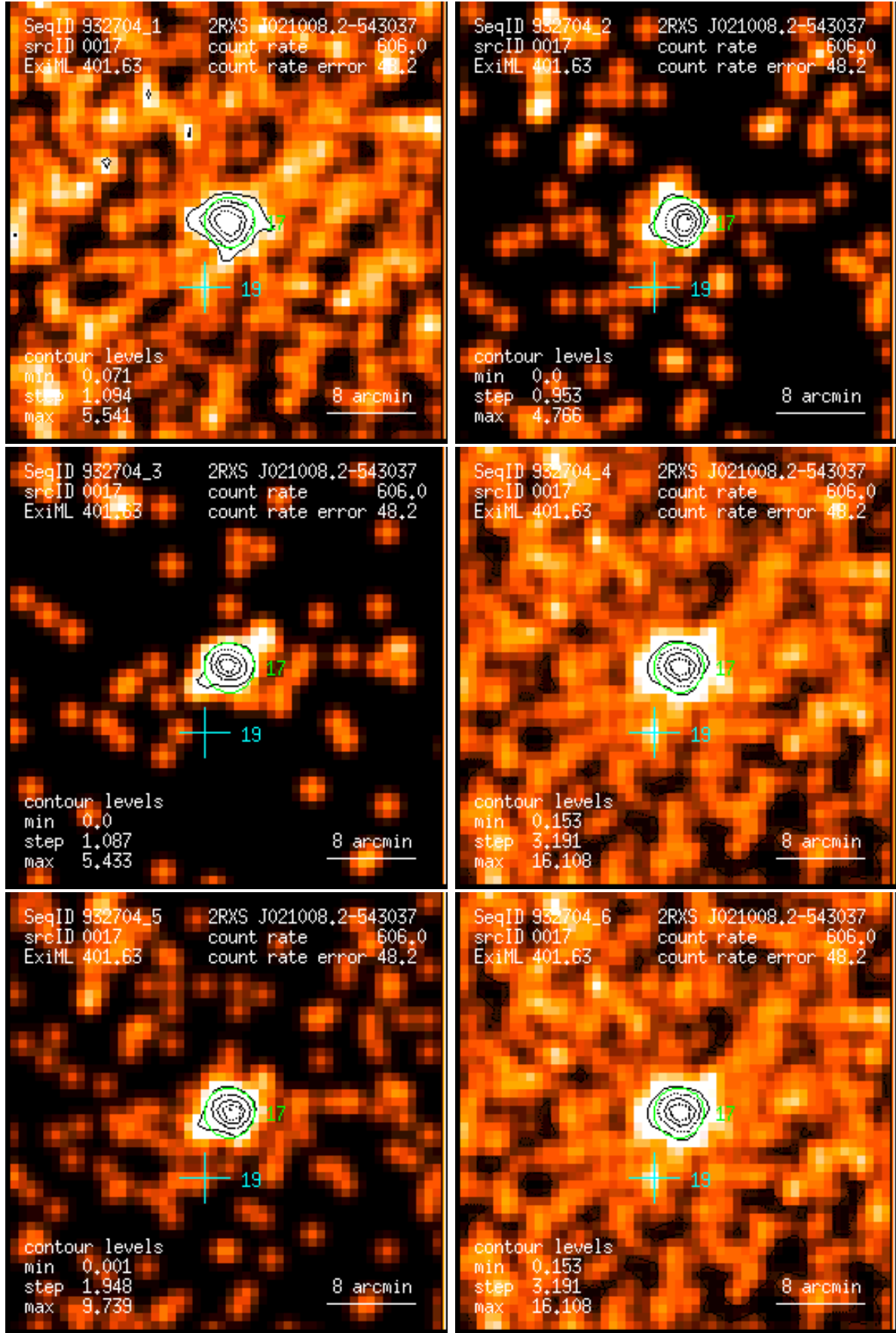
Figure 17: RASS 932704: detection 0017: band rate images, Gaussian filter: (1) PSPC channels 11 – 41, (2) 52 – 90, (3) 91 – 201, (4) 11 – 235, (5) 52 – 201, (6) 11 – 201. Broad band rates in counts/ks. Band rate contour levels in counts/ks/arcmin 2 .
