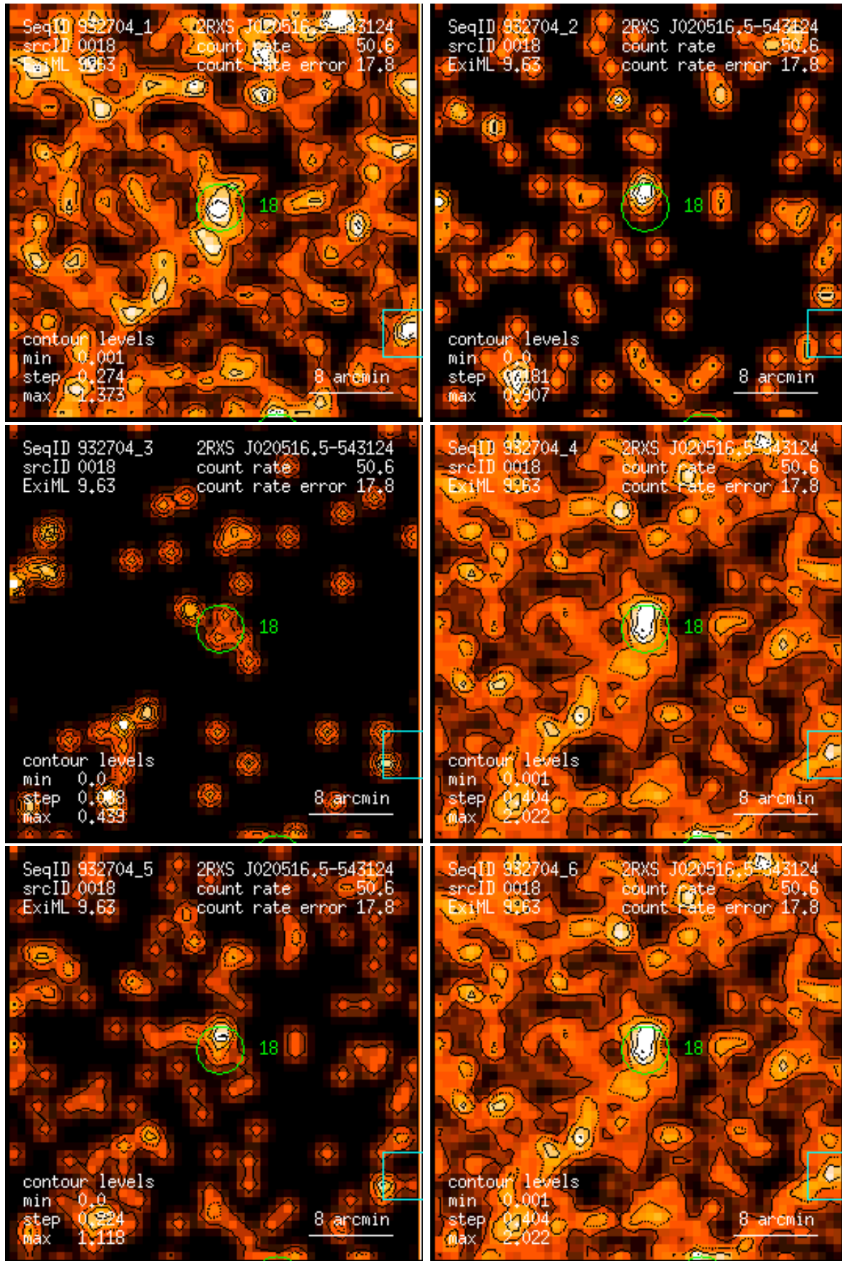
Figure 18: RASS 932704: detection 0018: band rate images, Gaussian filter: (1) PSPC channels 11 – 41, (2) 52 – 90, (3) 91 – 201, (4) 11 – 235, (5) 52 – 201, (6) 11 – 201. Broad band rates in counts/ks. Band rate contour levels in counts/ks/arcmin 2 .
