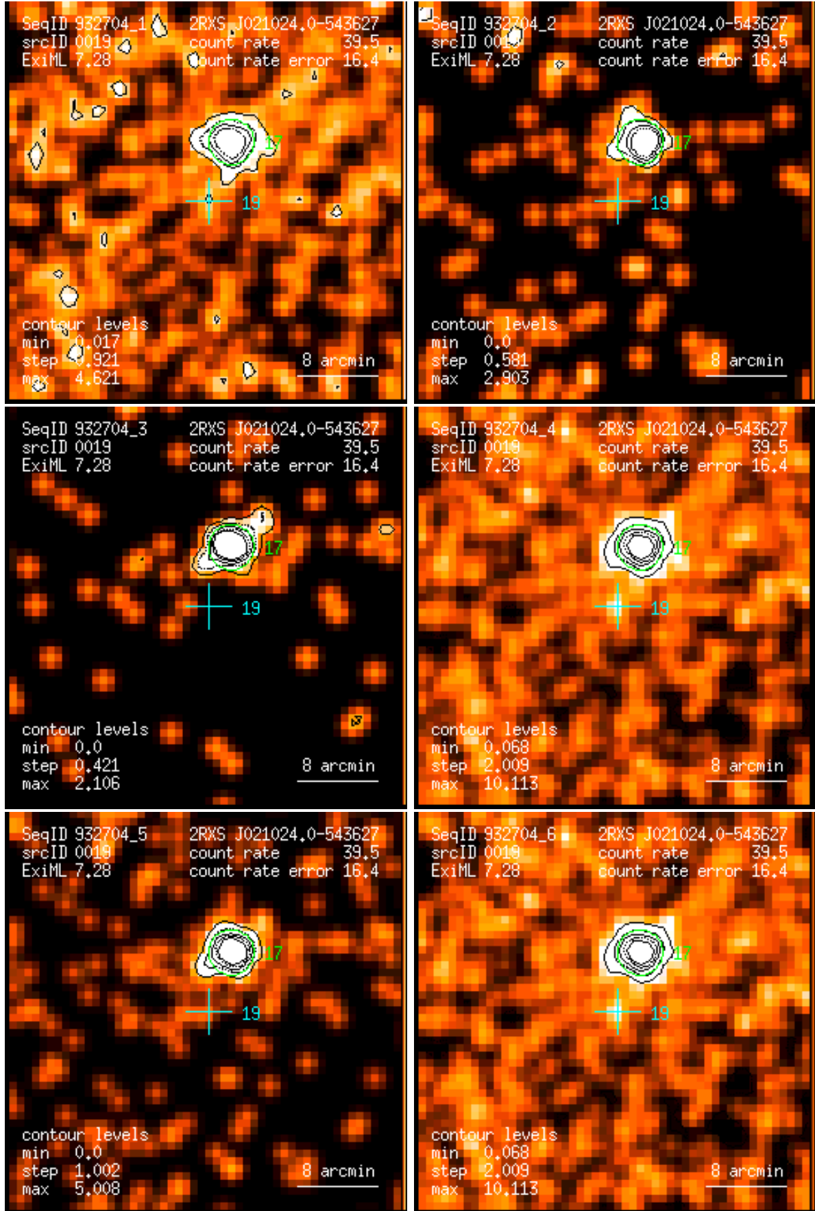
Figure 19: RASS 932704: detection 0019: band rate images, Gaussian filter: (1) PSPC channels 11 – 41, (2) 52 – 90, (3) 91 – 201, (4) 11 – 235, (5) 52 – 201, (6) 11 – 201. Broad band rates in counts/ks. Band rate contour levels in counts/ks/arcmin 2 .
