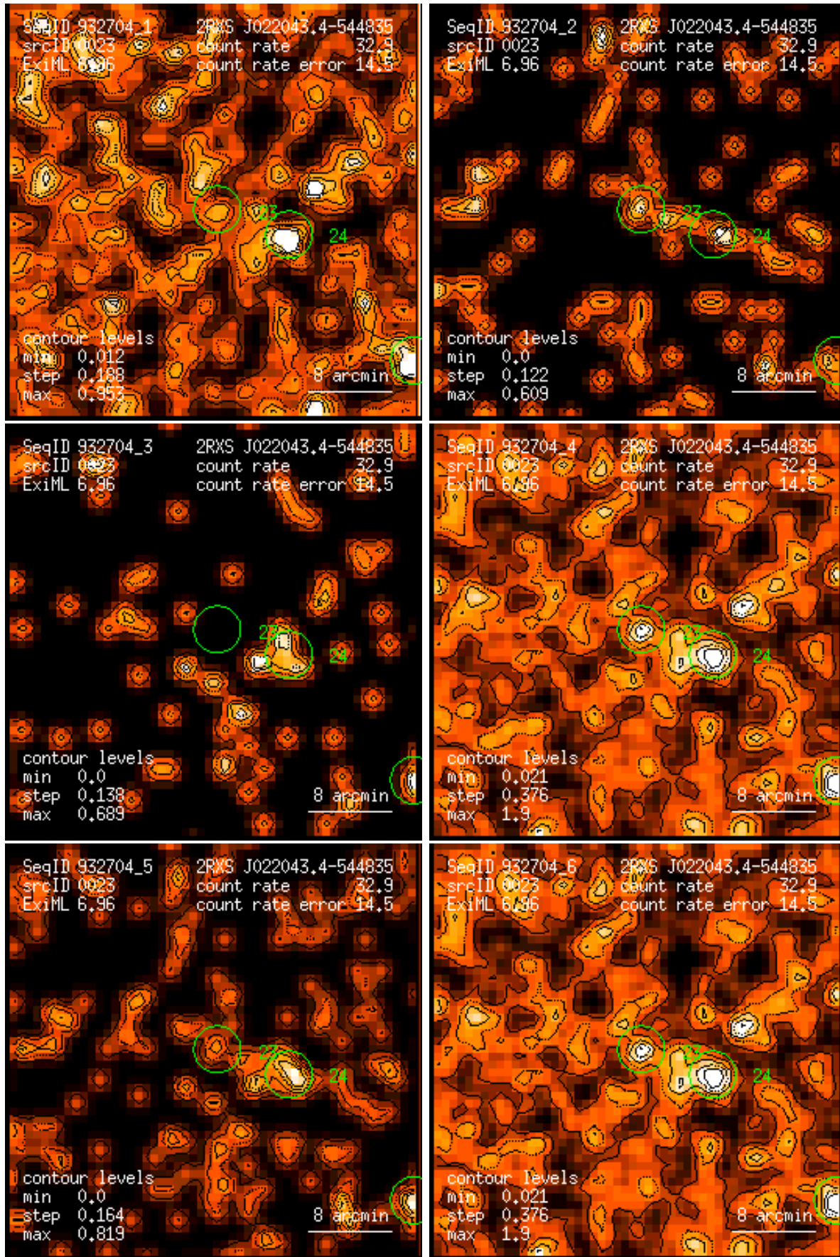
Figure 23: RASS 932704: detection 0023: band rate images, Gaussian filter: (1) PSPC channels 11 – 41, (2) 52 – 90, (3) 91 – 201, (4) 11 – 235, (5) 52 – 201, (6) 11 – 201. Broad band rates in counts/ks. Band rate contour levels in counts/ks/arcmin 2 .
