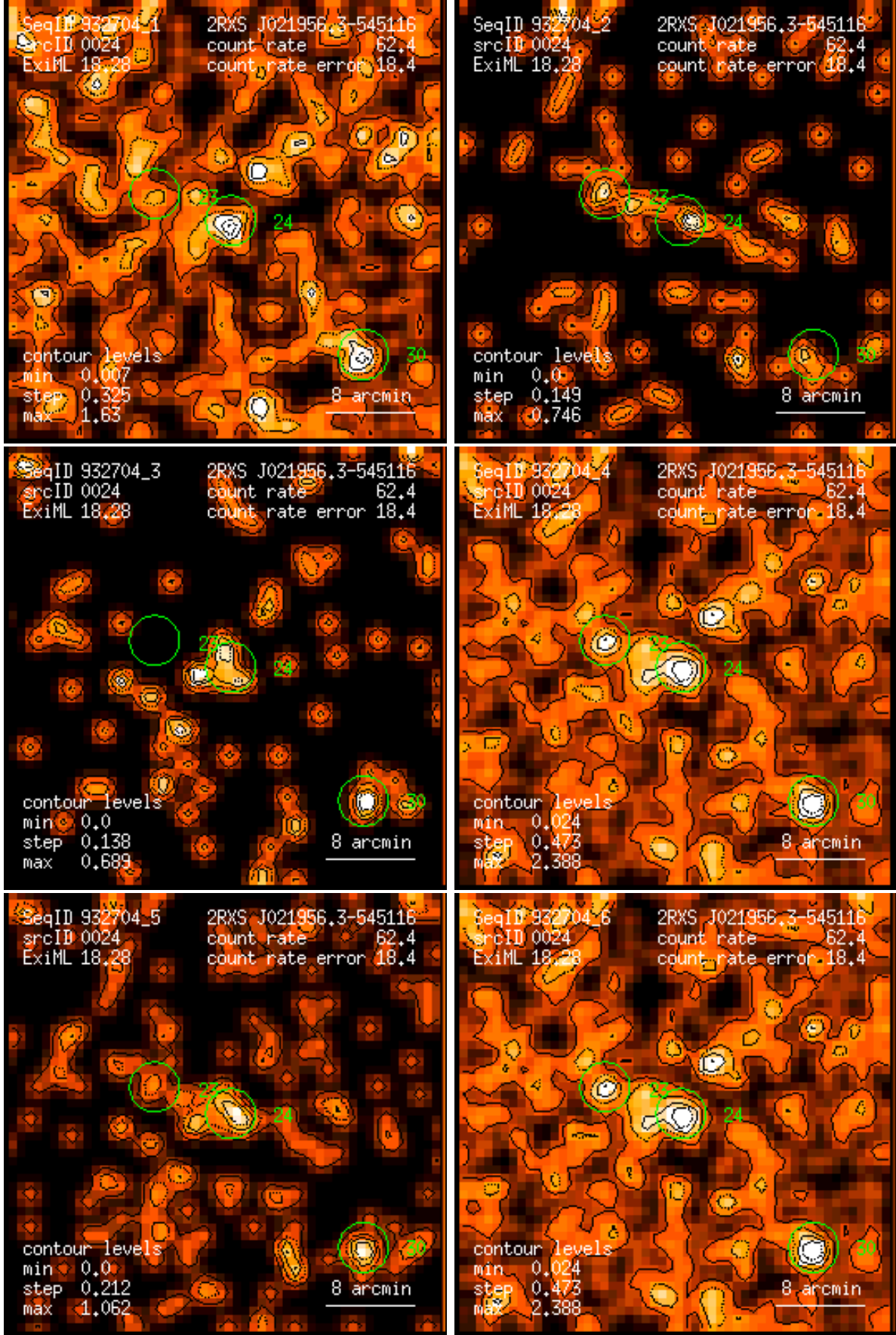
Figure 24: RASS 932704: detection 0024: band rate images, Gaussian filter: (1) PSPC channels 11 – 41, (2) 52 – 90, (3) 91 – 201, (4) 11 – 235, (5) 52 – 201, (6) 11 – 201. Broad band rates in counts/ks. Band rate contour levels in counts/ks/arcmin 2 .
