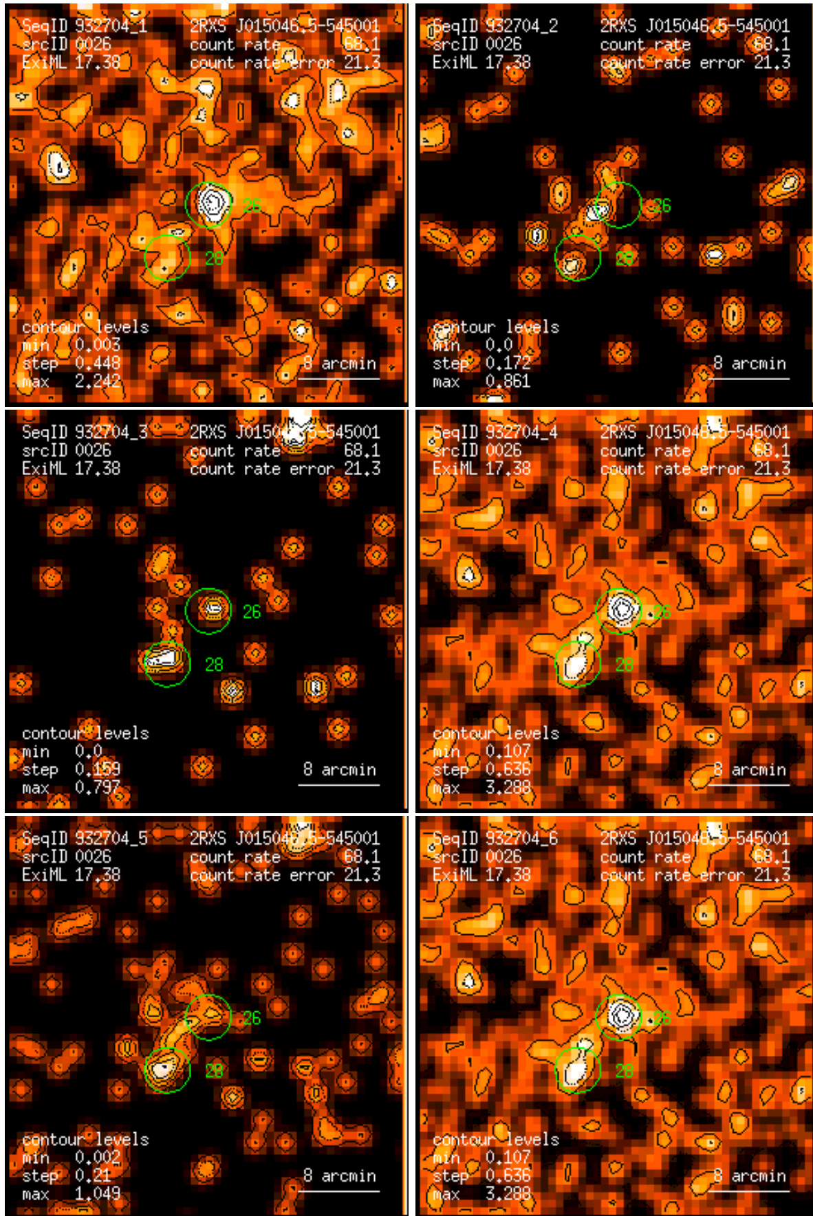
Figure 26: RASS 932704: detection 0026: band rate images, Gaussian filter: (1) PSPC channels 11 – 41, (2) 52 – 90, (3) 91 – 201, (4) 11 – 235, (5) 52 – 201, (6) 11 – 201. Broad band rates in counts/ks. Band rate contour levels in counts/ks/arcmin 2 .
