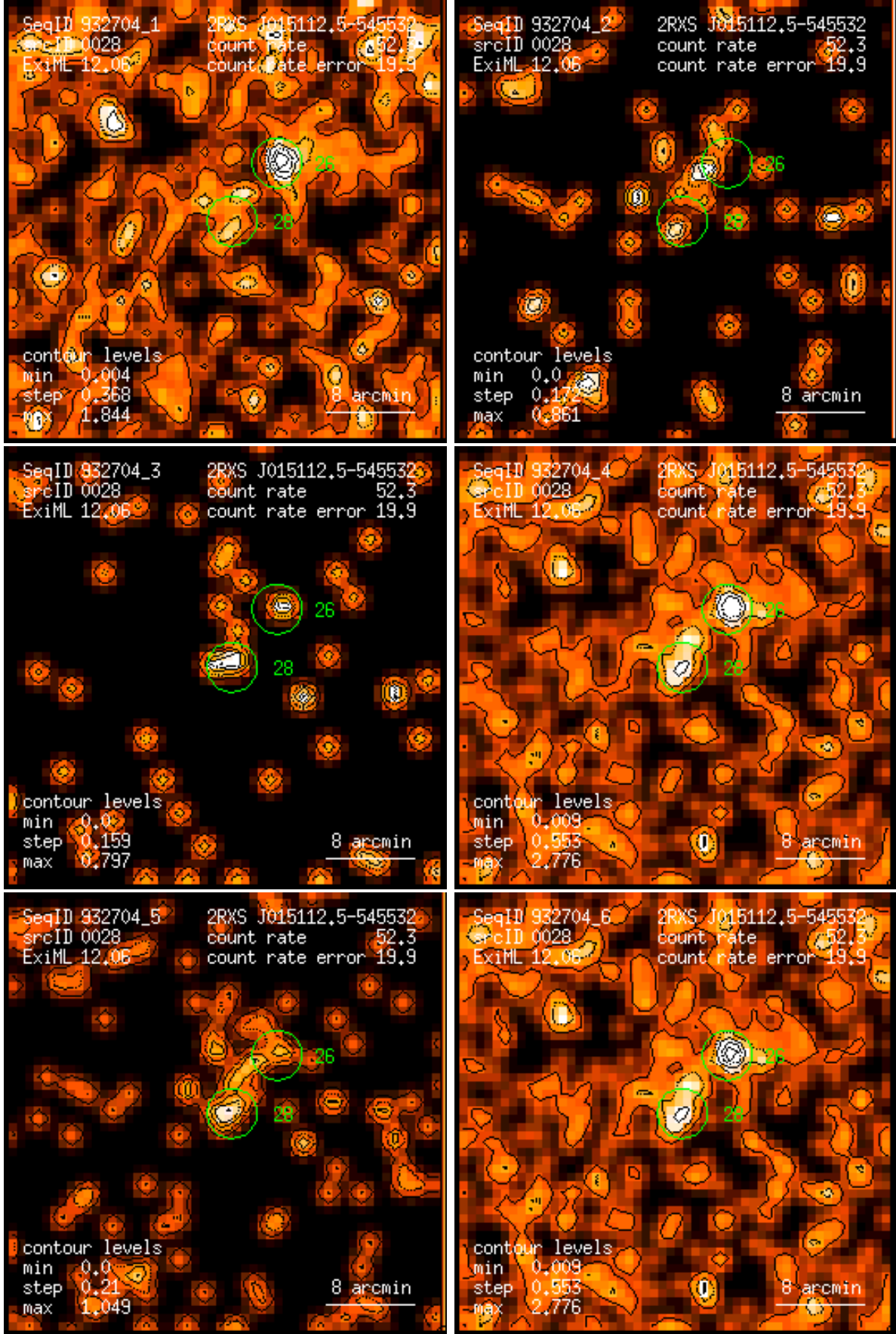
Figure 28: RASS 932704: detection 0028: band rate images, Gaussian filter: (1) PSPC channels 11 – 41, (2) 52 – 90, (3) 91 – 201, (4) 11 – 235, (5) 52 – 201, (6) 11 – 201. Broad band rates in counts/ks. Band rate contour levels in counts/ks/arcmin 2 .
