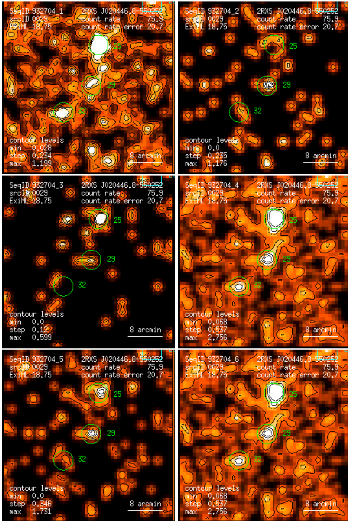
Figure 29: RASS 932704: detection 0029: band rate images, Gaussian filter: (1) PSPC channels 11 – 41, (2) 52 – 90, (3) 91 – 201, (4) 11 – 235, (5) 52 – 201, (6) 11 – 201. Broad band rates in counts/ks. Band rate contour levels in counts/ks/arcmin 2 .
