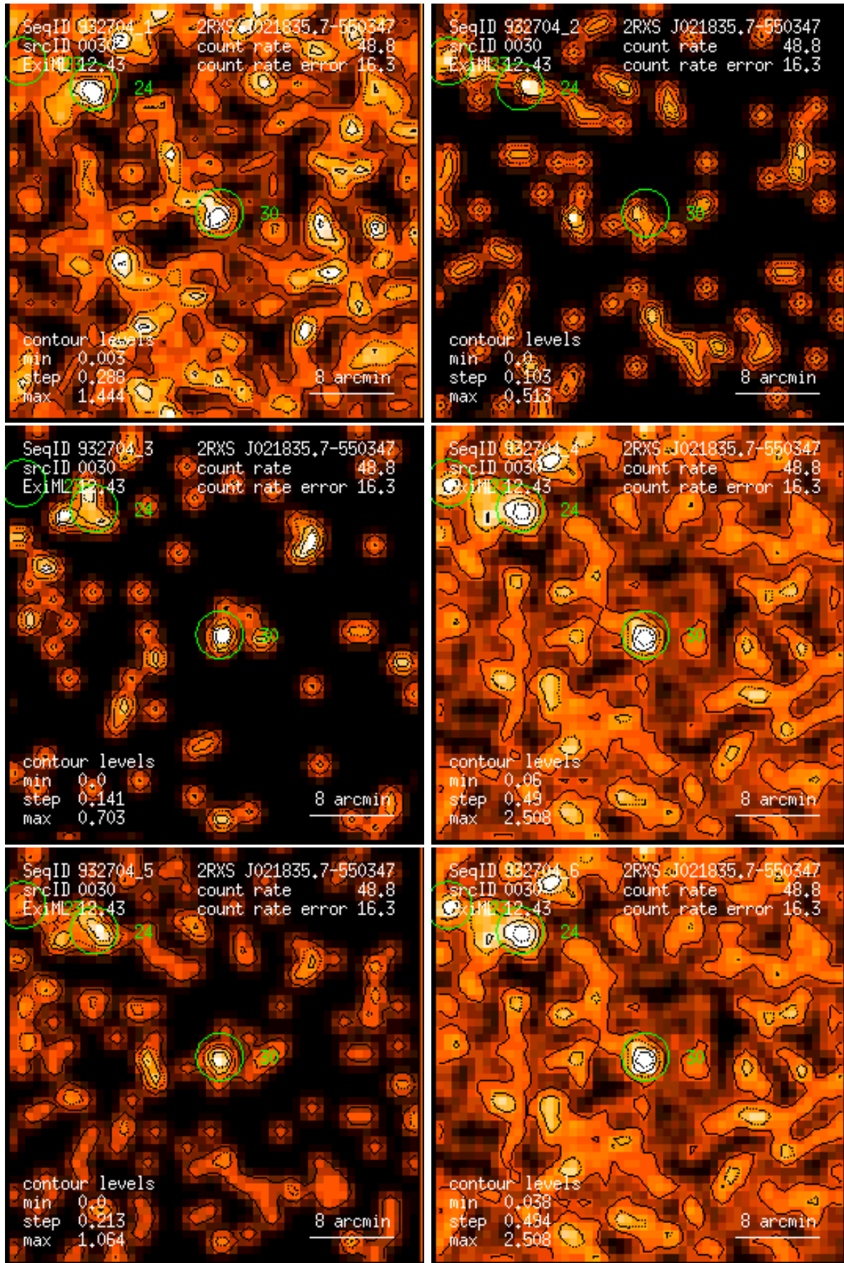
Figure 30: RASS 932704: detection 0030: band rate images, Gaussian filter: (1) PSPC channels 11 – 41, (2) 52 – 90, (3) 91 – 201, (4) 11 – 235, (5) 52 – 201, (6) 11 – 201. Broad band rates in counts/ks. Band rate contour levels in counts/ks/arcmin 2 .
