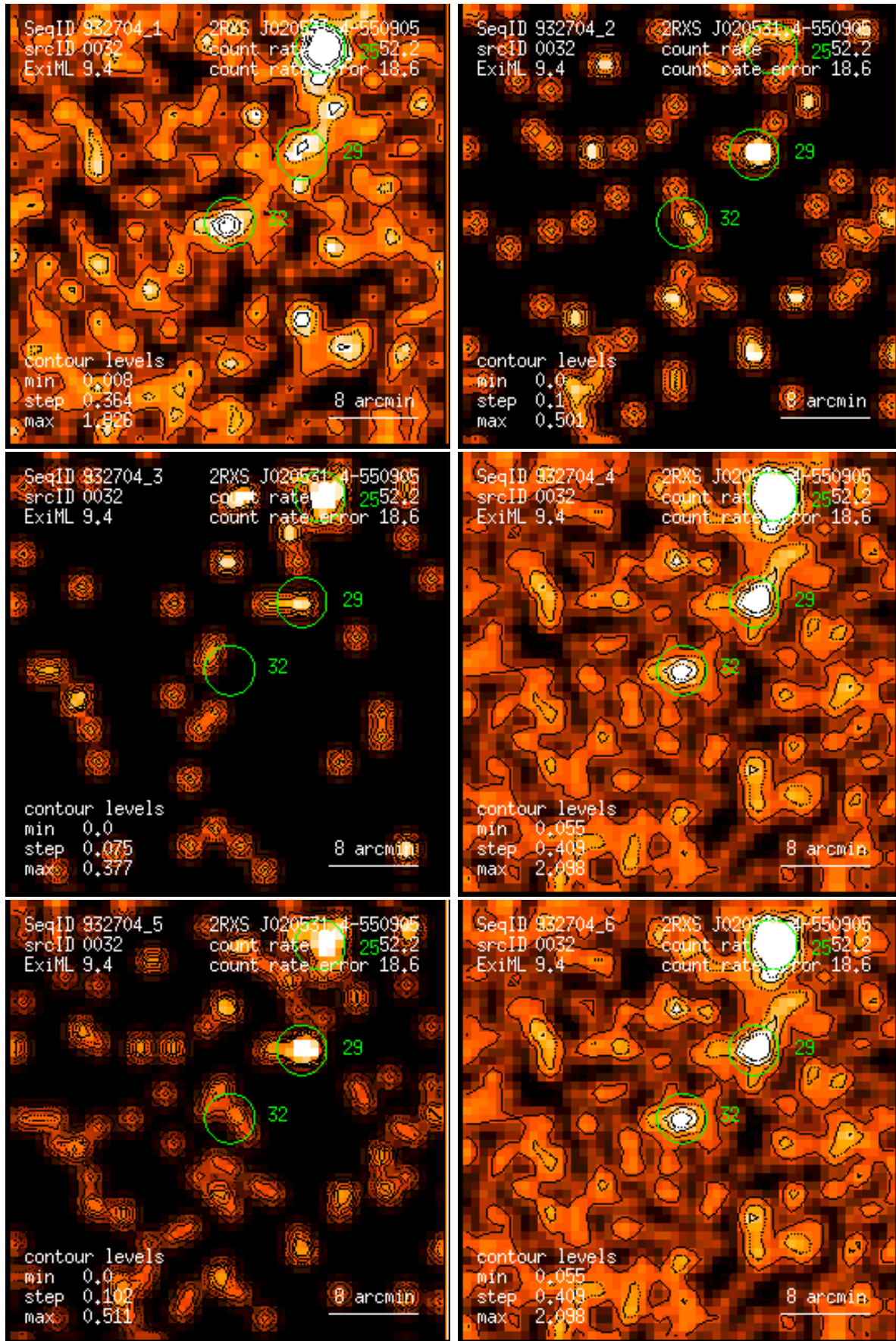
Figure 32: RASS 932704: detection 0032: band rate images, Gaussian filter: (1) PSPC channels 11 – 41, (2) 52 – 90, (3) 91 – 201, (4) 11 – 235, (5) 52 – 201, (6) 11 – 201. Broad band rates in counts/ks. Band rate contour levels in counts/ks/arcmin 2 .
