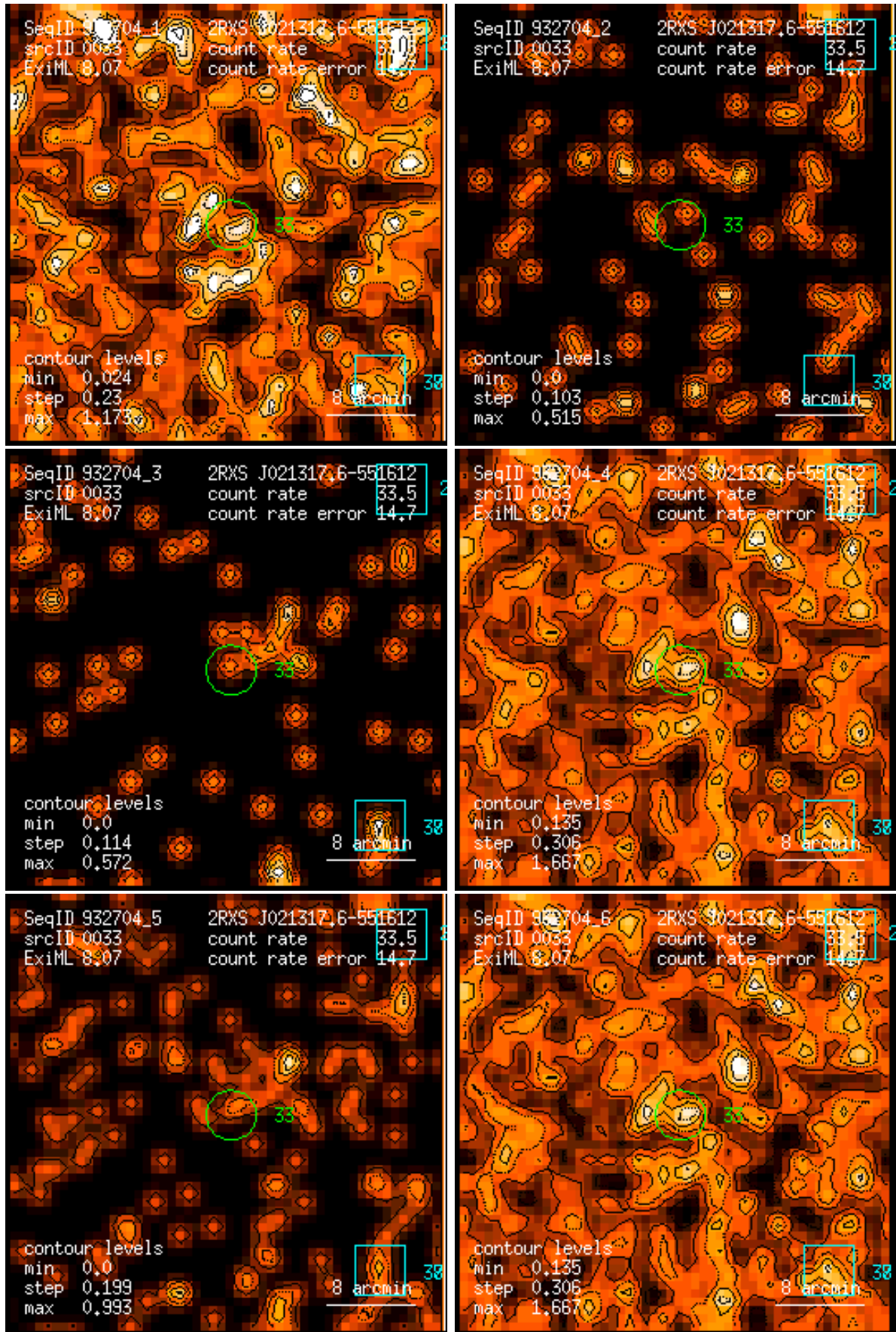
Figure 33: RASS 932704: detection 0033: band rate images, Gaussian filter: (1) PSPC channels 11 – 41, (2) 52 – 90, (3) 91 – 201, (4) 11 – 235, (5) 52 – 201, (6) 11 – 201. Broad band rates in counts/ks. Band rate contour levels in counts/ks/arcmin 2 .
